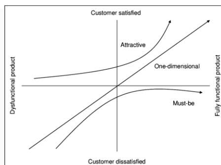
Gambar 1 Diagram Kano
