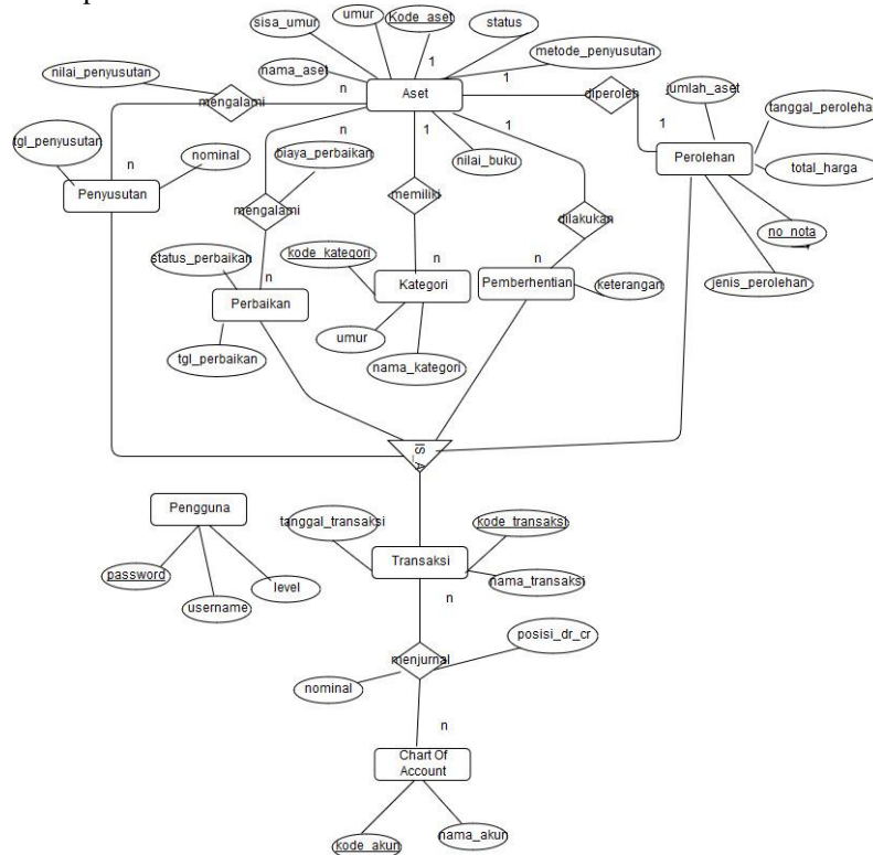
Gambar 3 Entity Relation Diagram
