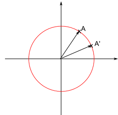
Fig. 3.4: Illustration of the rotation of the unit circle. For arbitrary rotations about the origin, all rotated points lie again in the initial set.
