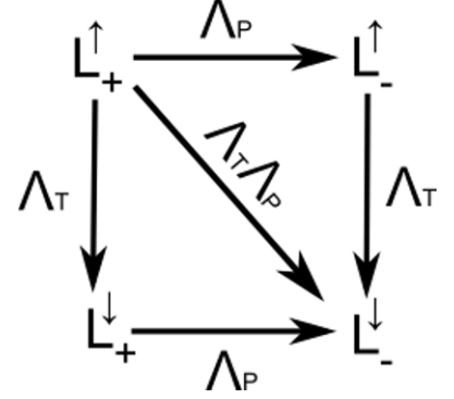
Fig. 3.8: The four components of the Lorentz group are connected through the two discrete transformations known as time-reversal \Lambda_T and space-inversion \Lambda_P .
