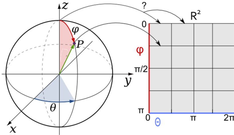
Fig. 3.9: Illustration of the map from one neighborhood of the sphere on to R^n .
