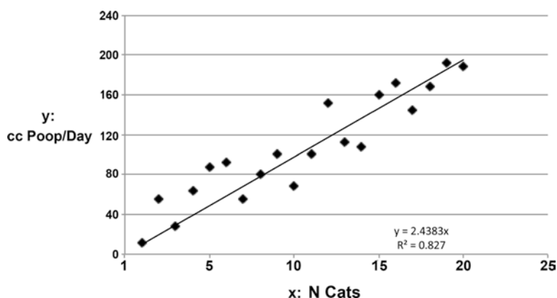
Fig. 18.4 A plot showing a distribution of variables with regression line, with formula for the intercept and R^2 (Illustration by the author)
