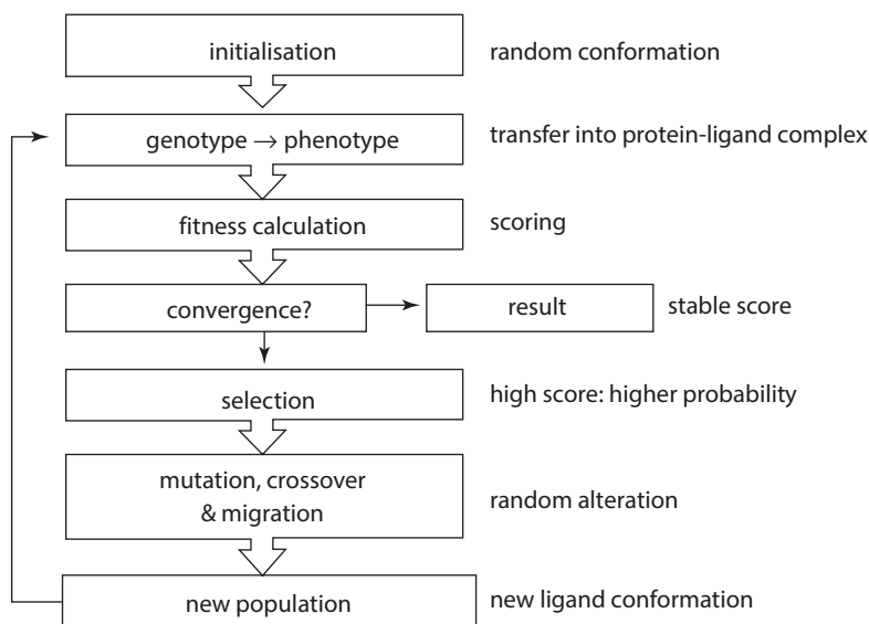
■ Fig. 5.7 Genetic algorithm used by docking software GOLD
