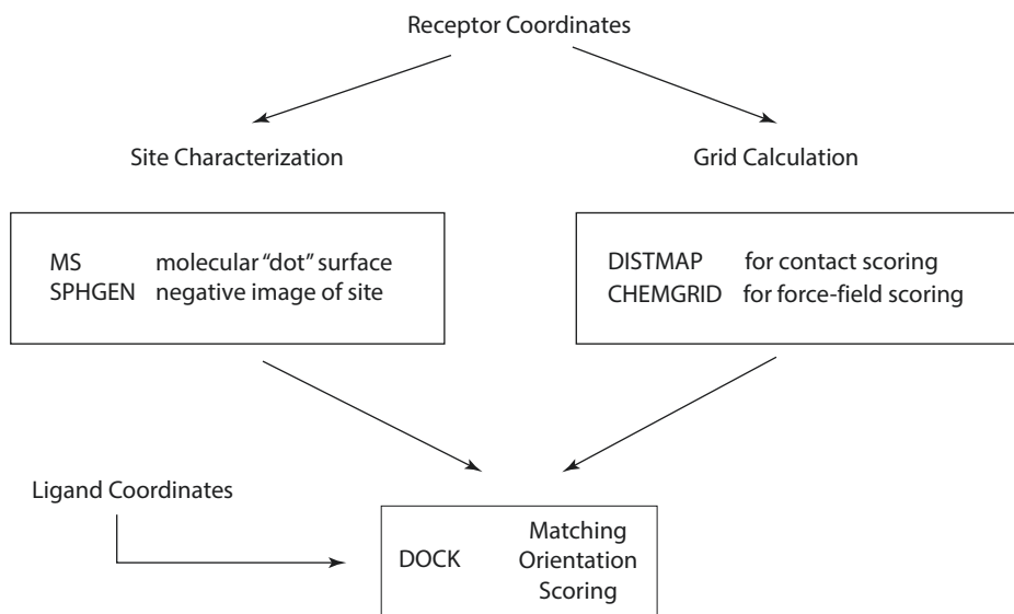
■ Fig. 5.4 Schematic representation of mode of operation of program DOCK [dock]
