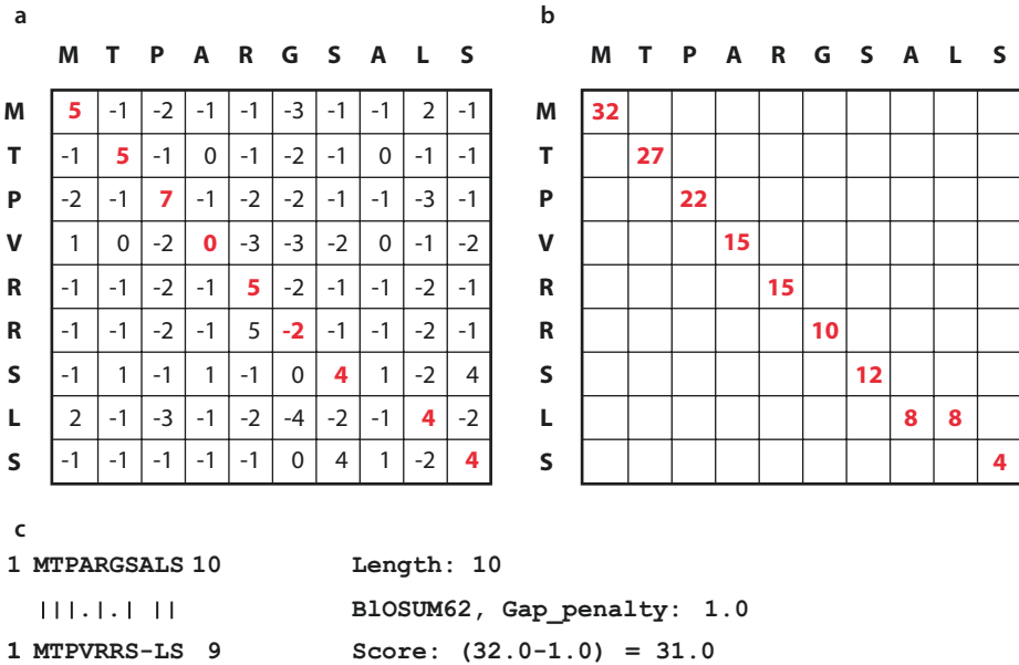
Fig. 3.4 Calculation of a global alignment of two similar protein sequences. a Both sequences are compared in a two-dimensional matrix, and the similarity of the amino acids is determined using similarity matrices. Each alignment can be described as a path through the two-dimensional matrix, starting with the highest-scoring amino acid pair at the N-terminus. b Adding the values produces corresponding scores for the different paths. The alignment with the highest score is considered optimal (red). c The optimal alignment is obtained by the introduction of a gap and contains 10 amino acids, of which 7 are identical. Using the BLOSUM62 similarity matrix and a gap penalty of 1.0 a score of 31.0 is achieved
