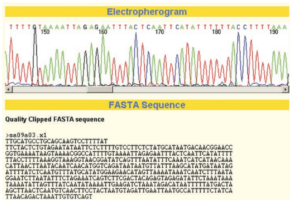
■ Fig. 4.1 Section of electropherogram from dideoxy DNA sequencing reaction with corresponding nucleotide sequence of expressed sequence tag (Clipping from Ensembl database, printed with kind permission from EBI, Hinxton, UK)
