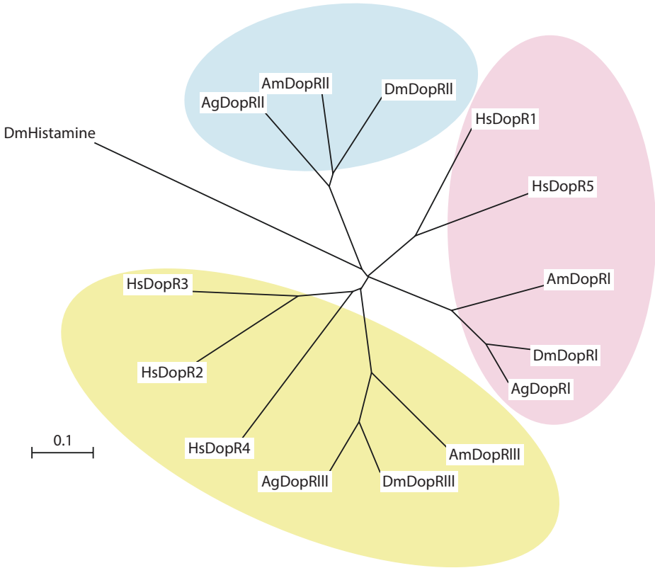
Fig. 3.6 Phylogenetic tree of dopamine receptor sequences. The evolutionary relationship between the sequences is reflected by the length of the branches. Dopamine receptor sequences of invertebrates ( Dm , Drosophila melanogaster ; Ag , Anopheles gambiae ; Am , Apis mellifera ) are compared with those of humans ( Hs , Homo sapiens ). Three clear clusters are formed. As a control, the phylogenetically distant sequence of the Dm histamine receptor was not found in any of the clusters
