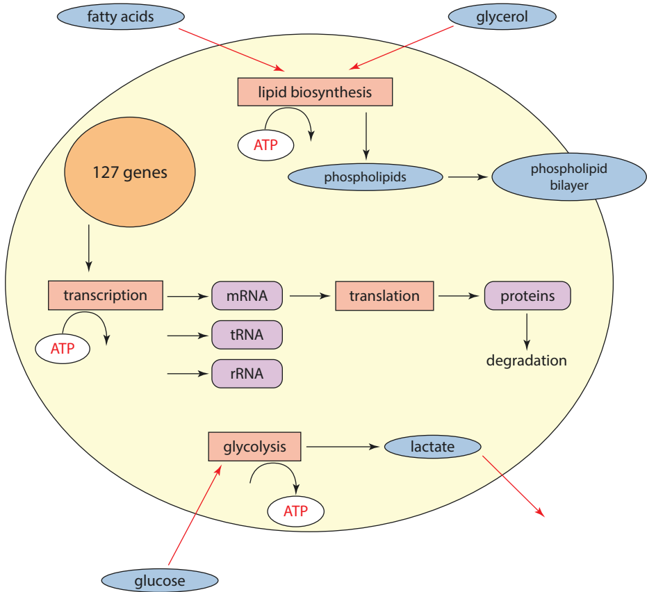
■ Fig. 6.15 Overview of metabolism in E-cell model. The model cell has pathways for glycolysis and phospholipid biosynthesis, transcription, and translation
