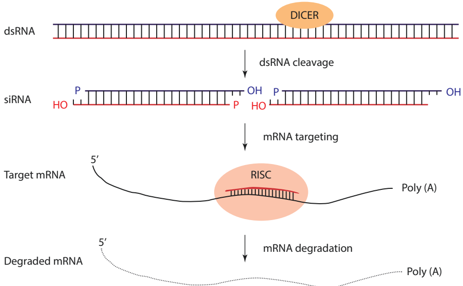
Fig. 6.13 Specific degradation of mRNA by RNA interference (RNAi). A type III ribonuclease (dicer) binds to and cleaves double-stranded RNA (dsRNA) into 21–25 base pair duplexes, termed small interfering RNA (siRNA). The siRNA is incorporated into the multiprotein complex called RNA-induced silencing complex (RISC), which also contains an RNase. RISC unwinds the siRNA, releases the sense strand, and facilitates hybridization of the antisense strand of the siRNA to the complementary strand of the cognate messenger RNA (mRNA). The binding activates the nuclease activity in the RISC, leading to cleavage of the target mRNA. The damaged mRNA is then degraded significantly, reducing the expression of the target gene
