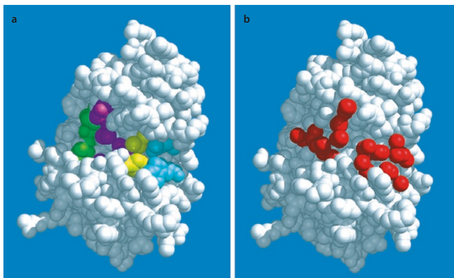
■ Fig. 5.5 Spherical model of cathepsin L-like cysteine protease of filarial Brugia pahangi . The underlying protein structure was generated by homology modeling. a The most important amino acids in the active site cleft, which is located between the two main domains of the protein, are indicated in color. The active site cysteine (top) and histidine (bottom) of the catalytic triad are highlighted in yellow. The active site asparagine is hidden in the structure. Important amino acids of the S' subunit are drawn in cyan, and those of the S subunit are in green and pink. b Graphical representation of characterization of catalytic cleft by DOCK program (subprogram SPHGEN). The centers of the overlapping spheres, where later the atoms of the ligands will lie, are represented in red
