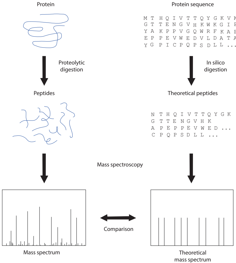
Fig. 6.7 Identification of proteins by cross-referencing data from mass spectrometry experiments and mass spectra that were theoretically computed
