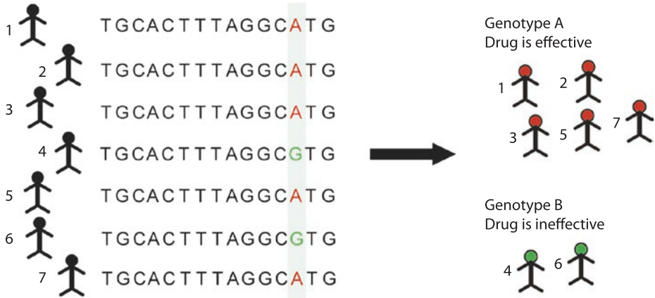
■ Fig. 4.9 Genotyping of patients by detecting SNPs
