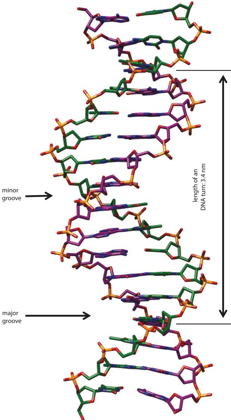
■ Fig. 1.2 Characteristic DNA double helix: B-DNA form containing major and minor grooves showing base pairs on the surface
