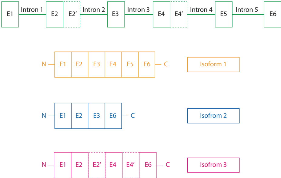
Fig. 4.7 Alternative splicing. The generation of several mRNA transcripts from a single gene by the combination of different exons (E) is called alternative splicing
