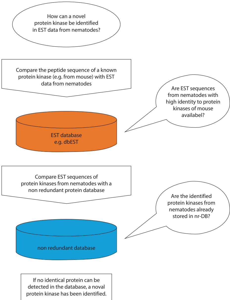
■ Fig. 4.6 Strategy for identification of new members of protein families
