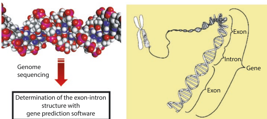
■ Fig. 3.9 Identification of new genes and proteins by genome sequencing
