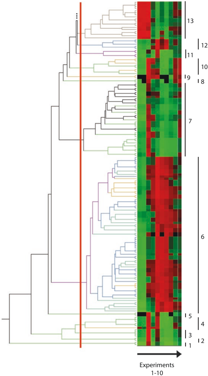
Fig. 6.4 Clustering of genes with similar expression profiles. Expression of 562 bacterial genes was measured in 10 different experiments. The expression profiles were then compared, and genes with similar expression patterns were grouped into clusters. In this figure, 13 clusters (black bars) with overall 164 genes are shown. For instance, cluster 13 contains 18 genes, which are highly expressed in the first 3 experiments (red), but then subsequently expression decreases (green). The red bar represents the threshold selected to define a cluster
