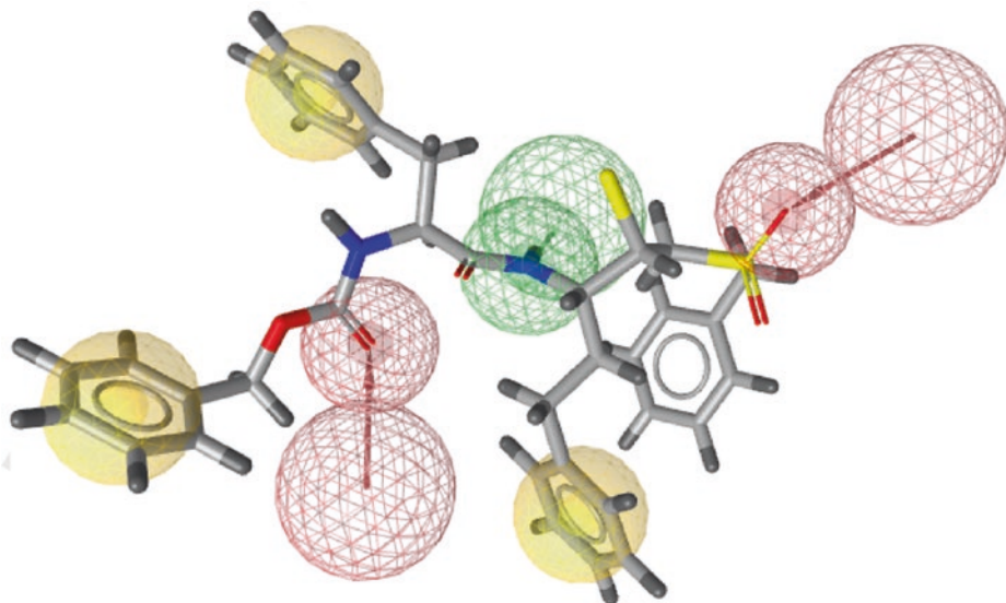
■ Fig. 5.9 Representation of a pharmacophore model. The pharmacophore features are shown as colored spheres. The shown properties are aromatic (yellow), hydrogen bond acceptor (red), and donor (green). A molecule fulfills this model when the pharmacophore features overlay with the pharmacophore model
