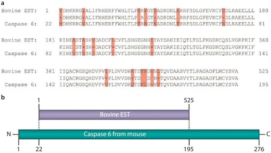
Fig. 4.4 Annotation of an EST sequence from bovine intestine. a The translated EST has an identity of 89% over a length of 175 amino acids (525 nucleotides) with murine caspase 6. Sequence differences are highlighted in red. The numbering of the EST sequence from 1 to 525 refers to nucleotides. In contrast, the numbering of the caspase 6 protein from 22 to 195 refers to amino acids. b Schematic of alignment of EST sequence with sequence of murine caspase 6
