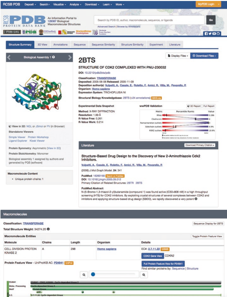
Fig. 2.10 Overview representation of PDB entry 2BTS (Printed courtesy of RCSB)
