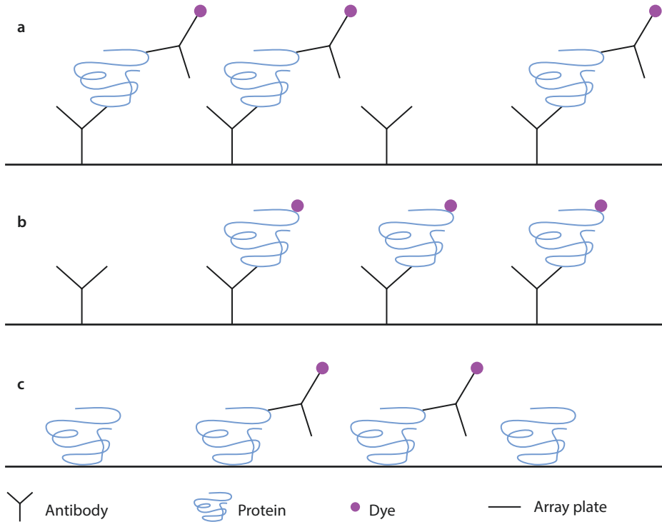
Fig. 6.10 Protein arrays. a In a sandwich assay, antibodies that are attached to array plates selectively bind to antigenic proteins after incubation with a protein lysate. Detection of the captured protein is performed with a secondary antibody that binds to a different antigenic site on the protein. b In an antigen capture assay, the antigenic proteins are labeled directly prior to incubation with the protein array, thereby dispensing with the need for a labeled secondary antibody for detection. c In direct or reverse-phase arrays, proteins are directly coupled to array plates and detected with labeled antibodies
