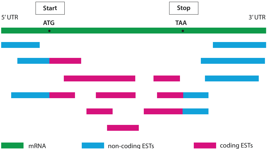
Fig. 4.5 EST sequences are derived from coding and noncoding segments of an mRNA
