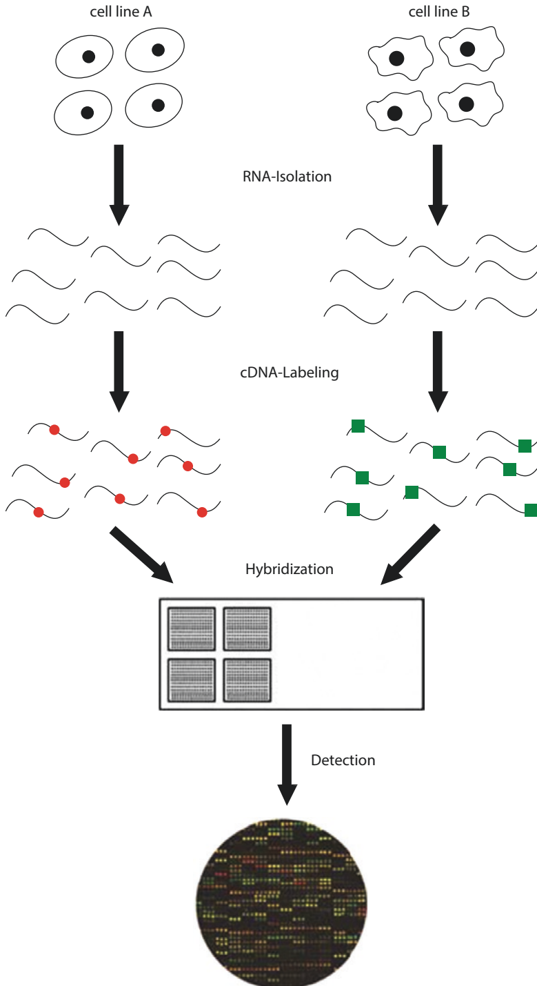
Fig. 6.3 Comparison of gene expression levels in two different cell lines as part of an expression profiling experiment using cDNA microarrays (Iron chip, printed with permission from M. Muckenthaier, EMBL Heidelberg, Germany)
