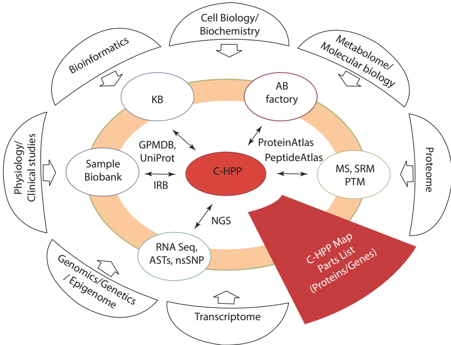
■ Fig. 6.5 Chromosome-based part of the Human Proteome Project (C-HPP). MS: mass spectroscopy, AB: antibody, KB: knowledge base (Taken from ► http://www.c-hpp.org/ )
