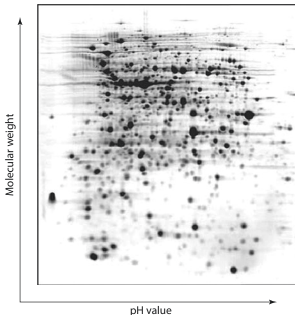
Fig. 6.6 Two-dimensional polyacrylamide gel electrophoresis (2D-PAGE). A protein lysate of a bacterium was separated along a pH gradient (pH 3–10) in the first dimension and by molecular mass in the second dimension. The resolved proteins were then visualized by silver staining
