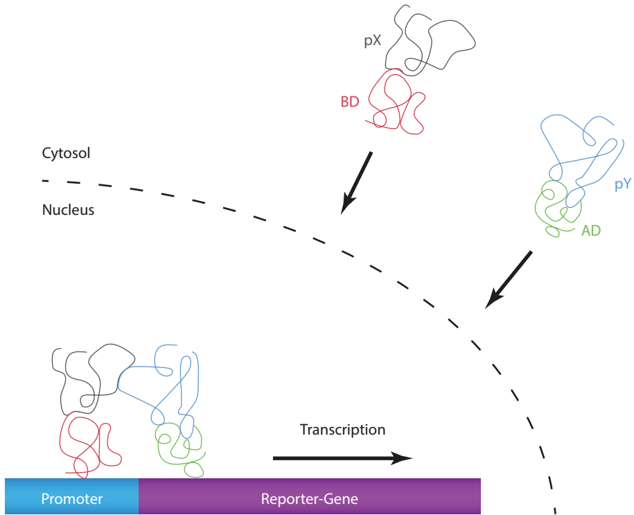
Fig. 6.9 Identification of protein–protein interactions using yeast two-hybrid system. Transcription of a reporter gene can only be activated when a fusion protein composed of the DNA binding domain of a transcription factor (BD) and a random protein X (pX) interact with a second fusion protein containing the cognate transcription factor’s activating domain (AD) and a random protein Y (pY)
