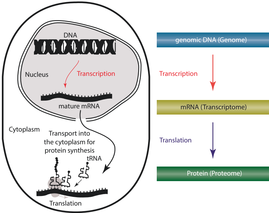
Fig. 1.4 The central dogma of molecular biology. The flow of information always proceeds from the genome to the proteome, not vice versa. Exceptions are reactions that are catalyzed by the reverse transcriptase and replicase of RNA viruses
