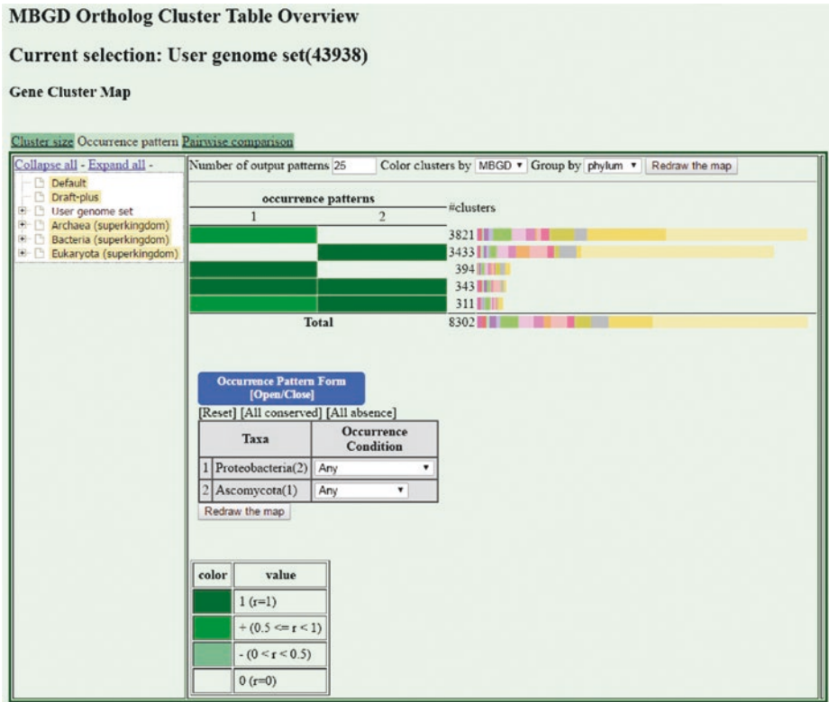
Fig. 7.8 Result of a cluster analysis of the MBGD [mbgd]. The organisms E. coli (Ecs), H. pylori (Hpj), and S. cerevisiae (Sce) were selected for calculating the underlying cluster table (Printed courtesy of MBGD)
