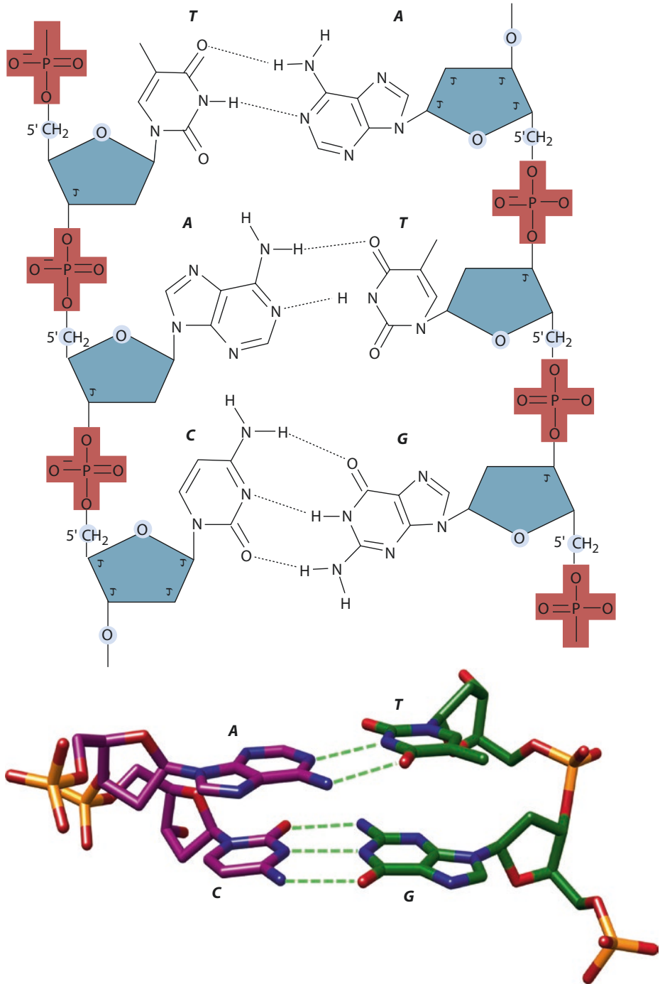
Fig. 1.1 The composition of nucleic acids: a schematic representation; b DNA double helix cutout with both possible pairings: adenine-thymine (A-T) and cytosine-guanine (C-G)
