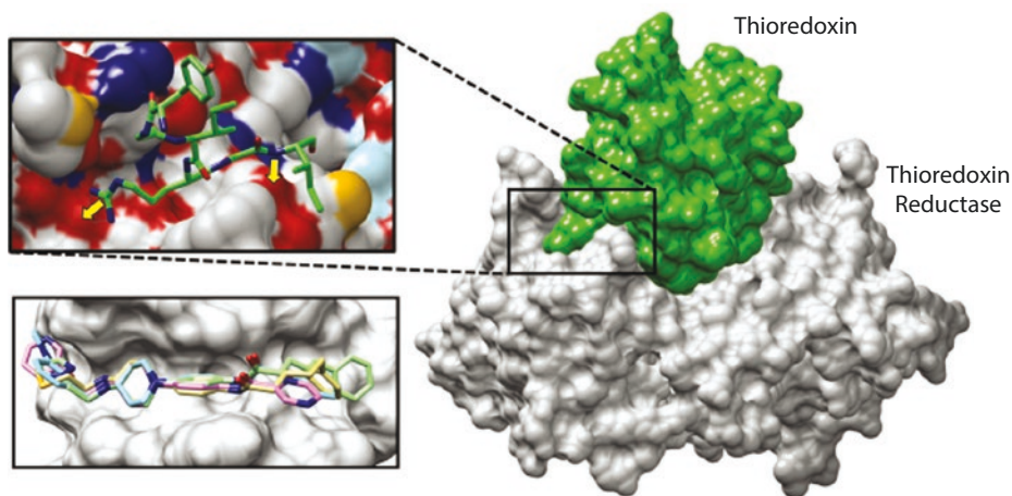
Fig. 5.8 Thioredoxin reductase (gray) and its substrate thioredoxin (green). The top cutout shows the target point for the docking-based virtual screening (yellow arrows: hydrogen bonding interaction). The bottom cutout shows the docking poses of four inhibitors sharing a common scaffold
