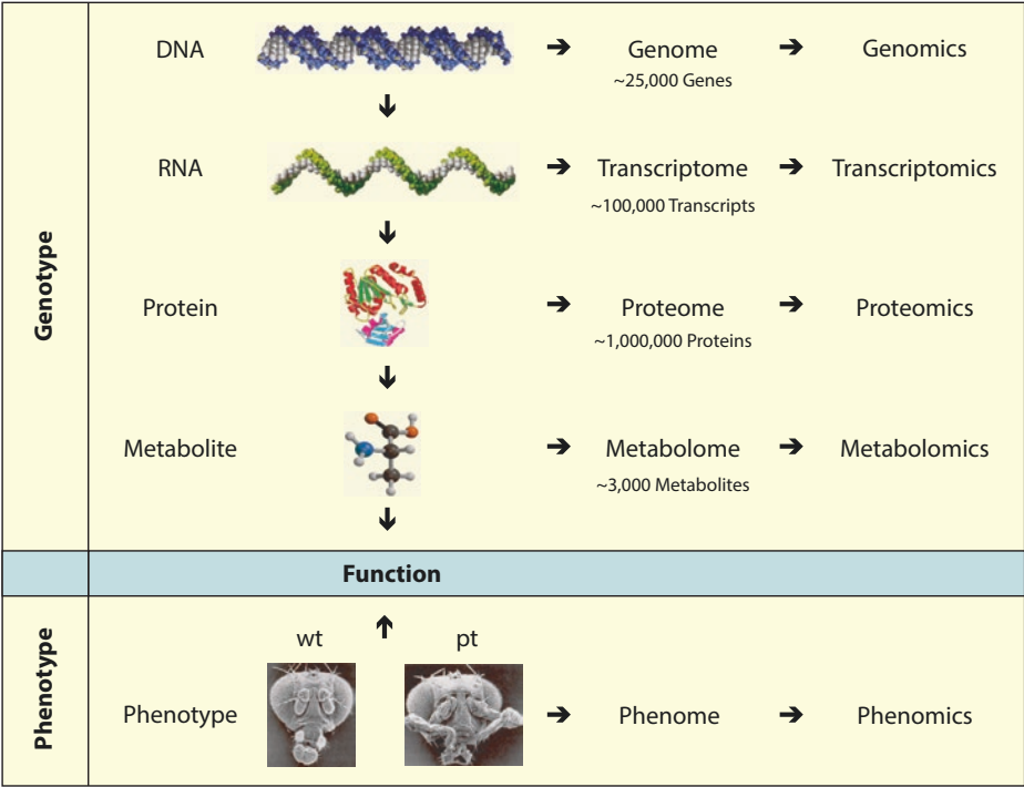
Fig. 6.1 Correlation between genotype and phenotype. From the genome via the transcriptome, proteome, and metabolome to the phenome. The example numbers in the genotype section are taken from Homo sapiens . The example in the phenotype section is taken from Drosophila melanogaster (Graphics of DNA, RNA, and metabolite from Lehninger Biochemie , 3rd Edition 2001, printed with permission from Springer-Verlag, Heidelberg, Germany. D. melanogaster microscopy images printed with permission from F. Rudolf Turner of Indiana University)
