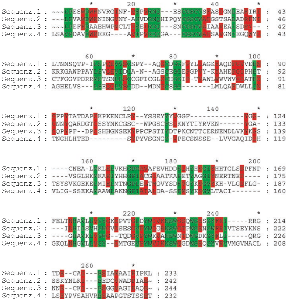
Fig. 3.5 Multiple-sequence alignment of four related proteins. Amino acids conserved in all four sequences (or with conservative changes) are highlighted in green; those conserved only in three of four sequences are shaded red
