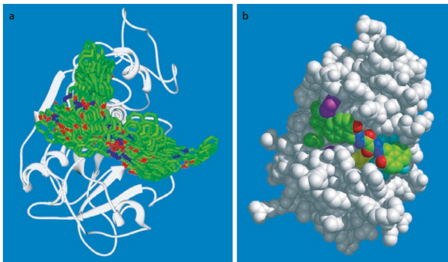
■ Fig. 5.6 Model of catalytic cleft of cathepsin L-like cysteine protease of Brugia pahangi , into which a chemical compound was modeled using DOCK. a The protein is displayed in its secondary structure (ribbon model). In single DOCK mode, all possible orientations of a chemical compound (hydrazide) were generated. All overlapping orientations of this single compound are represented in the figure: carbon, green; oxygen, red; nitrogen, blue. b Based on the analysis of the docking experiment described in panel a , the most likely orientation of the hydrazide in the catalytic cleft of the cysteine protease is shown. Protein and chemical compounds are represented as spheres. Coloration is similar to those in panel a and ■ Fig. 5.5
