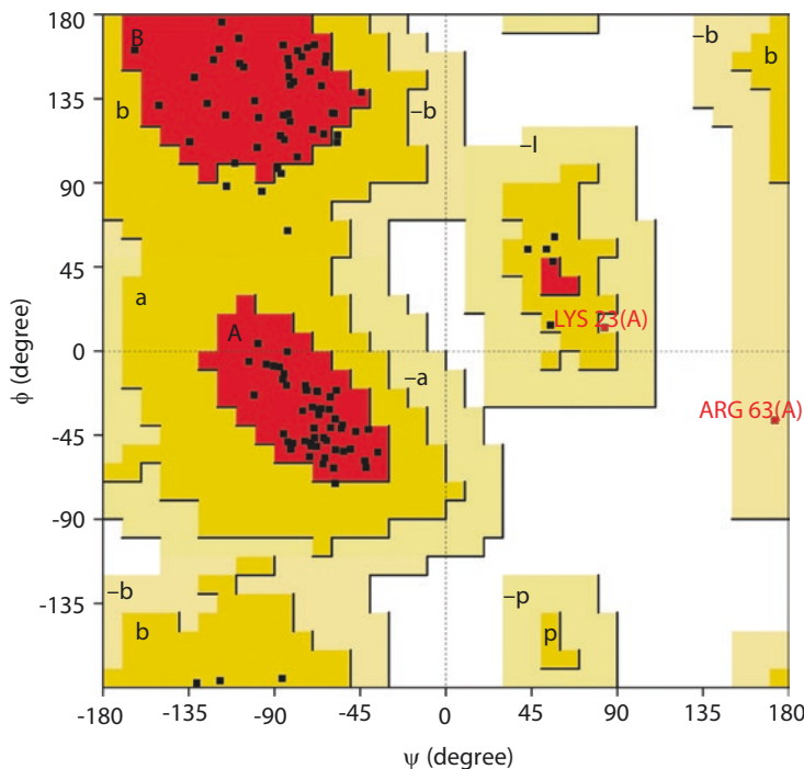
Fig. 1.8 Ramachandran plot of transcription regulator protein GAL4 from Saccharomyces cerevisiae . The amino acids are represented as small black squares. Evidently almost all amino acids lie in preferred, permissible areas (red and yellow). Two amino acids (LYS23 and ARG63) are found in slightly forbidden areas of the Ramachandran plot. This means that the combination of the values for \psi and \phi would theoretically not be possible owing to the steric hindrance of the neighboring side chains. However, in practice, it can be observed. The plot was generated with the program PROCHECK (Laszkowski et al. 1993; Rullmann 1996); plot statistics were deleted for clarity
