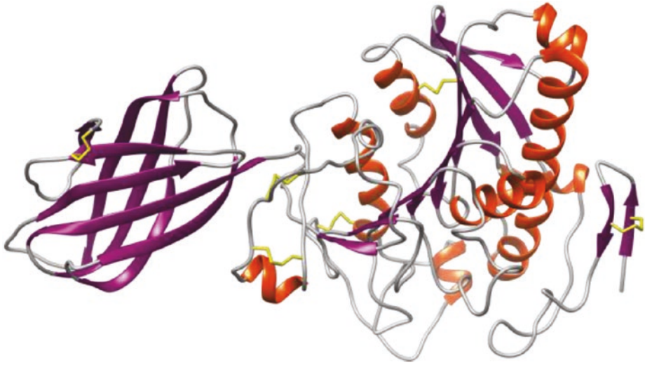
■ Fig. 1.9 Secondary structure representation (ribbon model) of a horse pancreas lipase with two domains (left: only \beta -sheets, right: \alpha -helices and \beta -sheets). Orange coils symbolize \alpha -helices and purple arrows \beta -strands. The connections between these are loop regions that consist of turns. Disulfide bridges, which stabilize the three-dimensional structure of the protein, are represented in yellow
