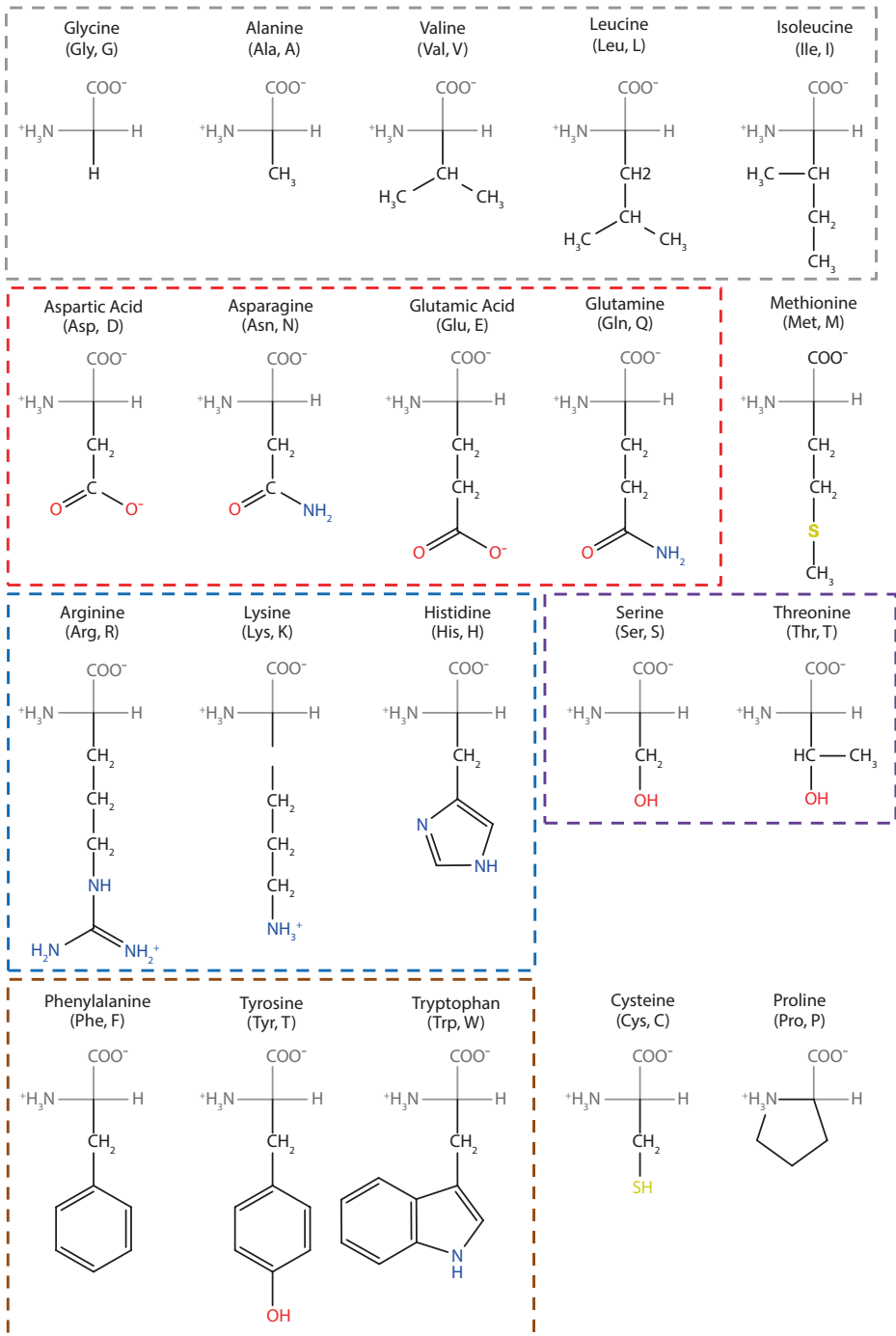
Fig. 1.6 The main L-amino acids with three-letter and one-letter codes. The colored lines group amino acids with similar properties: aliphatic side chains (gray), acids and their amides (red), basic side chains (blue), with a hydroxyl group (magenta) and aromatic side chains (orange)
