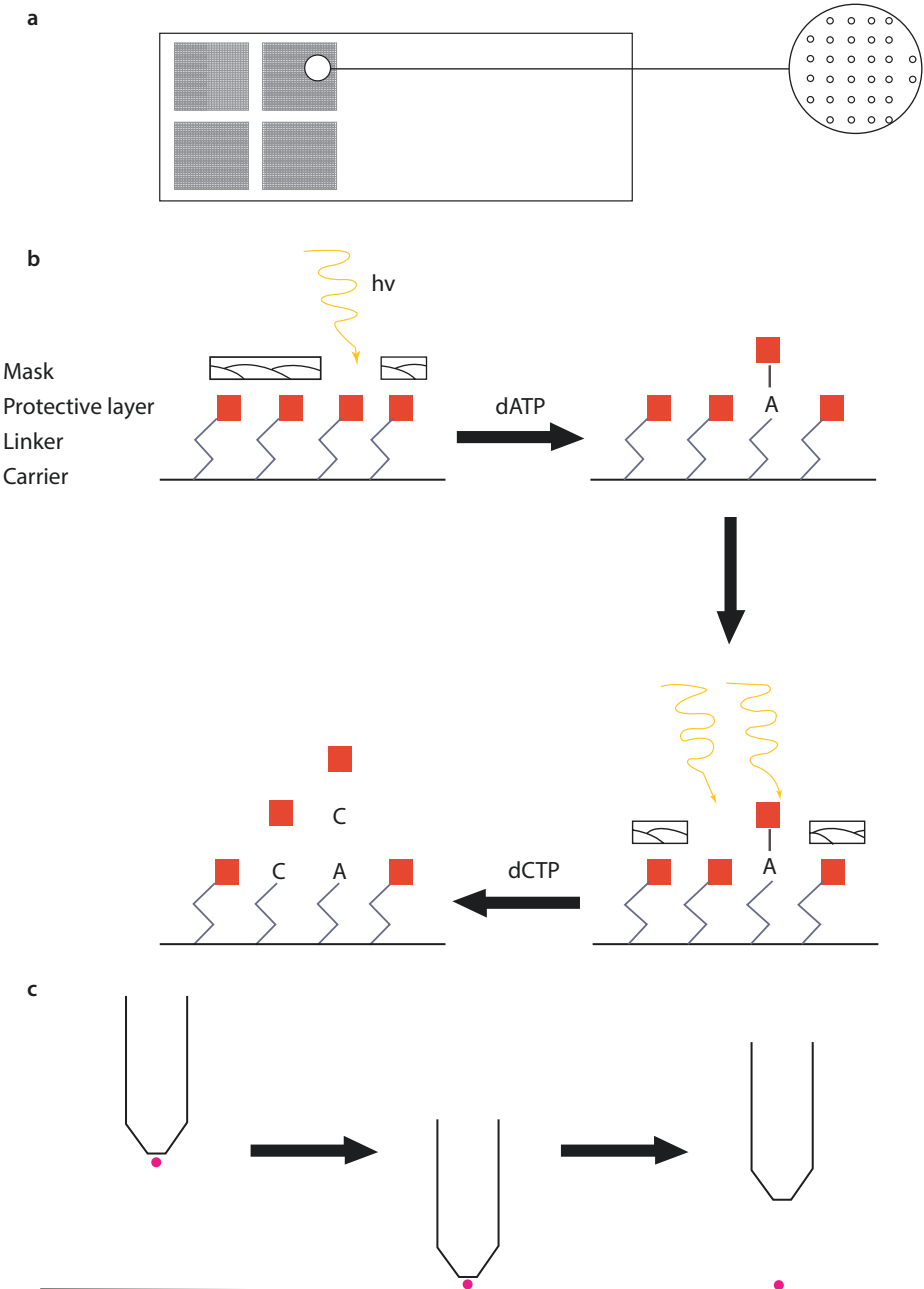
Fig. 6.2 DNA microarrays. a DNA microarray that consists of several thousand nucleic acid spots and arrayed in high density. b Schematic illustration of production of an oligonucleotide array using photolithography. c cDNA solutions are spotted during array production onto microarray plates by robots
