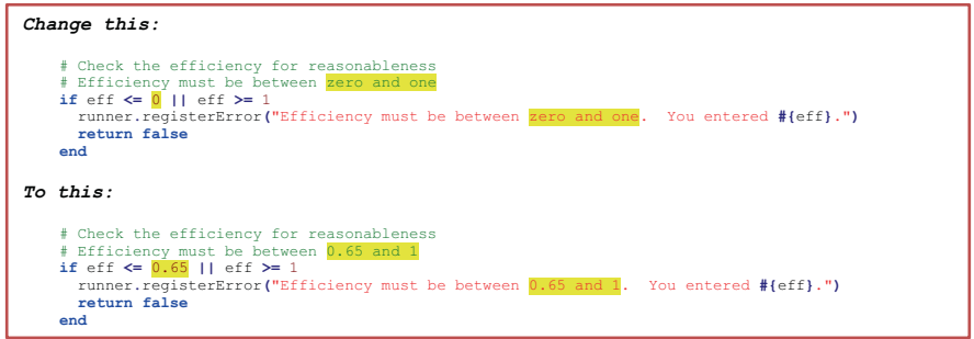
Fig. 9.12 Making a second change to the Measure
