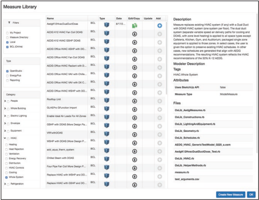
Fig. 6.47 Downloading the AEDGK12HVACDualDuctDoas Measure
