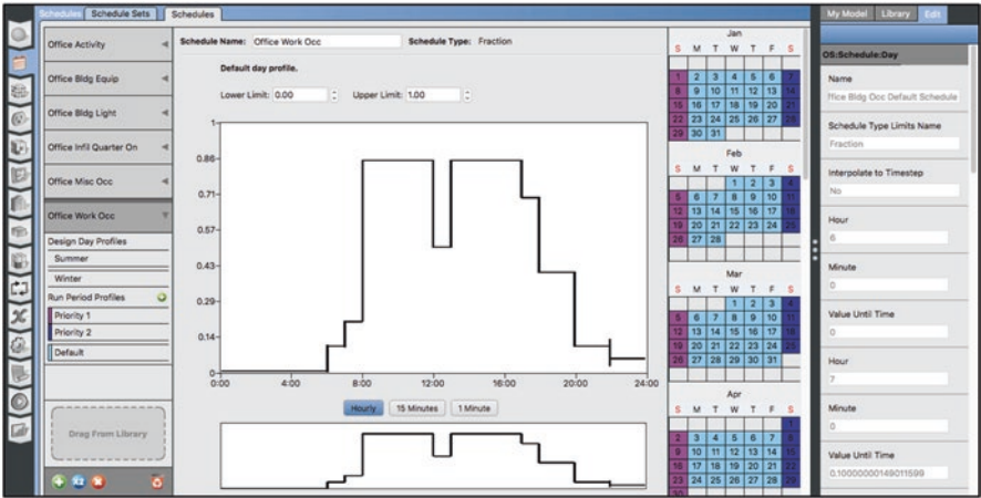
Fig. 3.3 An office Ruleset Schedule defined for weekdays
