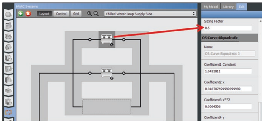
Fig. 5.28 Sizing factor used for components installed on branches
