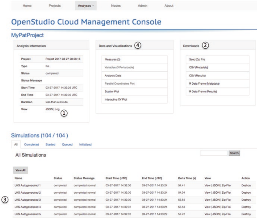
Fig. 7.33 OpenStudio Cloud Management Console view of a project
