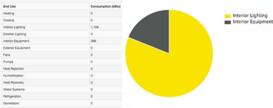
Fig. 3.40 Annual end use breakdown for Bob's Unconditioned Office
