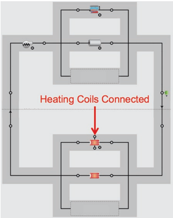
Fig. 5.50 Hot Water Loop with Heating Coils connected
