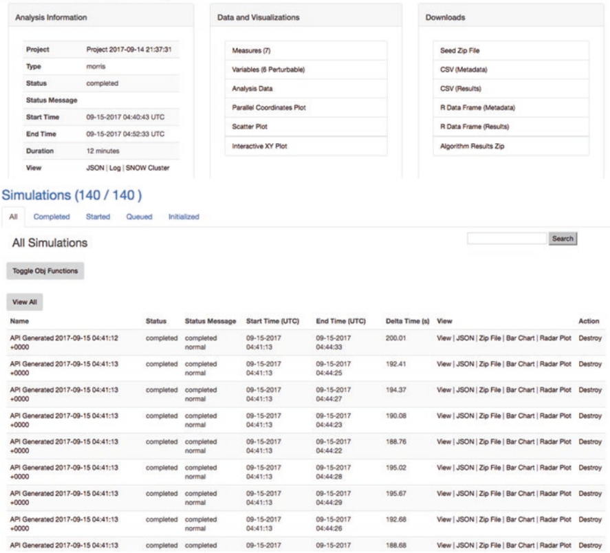
Fig. 7.50 Completed Morris Method analysis for school model problem
