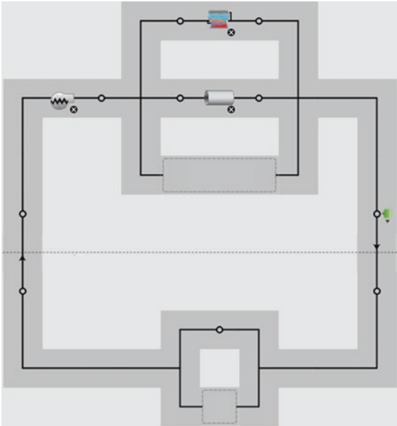
Fig. 5.49 Hot Water Loop with initial components
