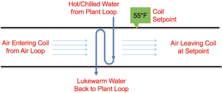
Fig. 5.25 Air and Water Flow through a Coil
