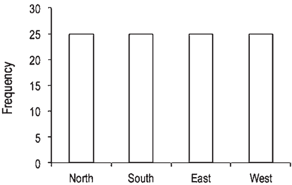
Fig. 7.14 Discrete distribution for cardinal direction
