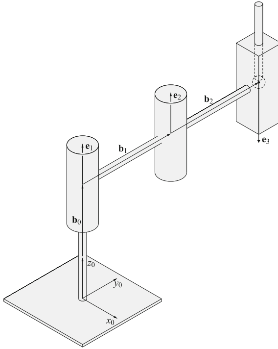
Fig. 3.7 The SCARA robot manipulator in the initial pose
