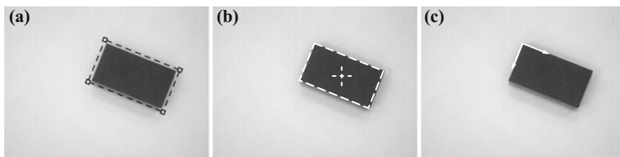
Fig. 8.8 a Model definition, b recognized object's features, c located object
