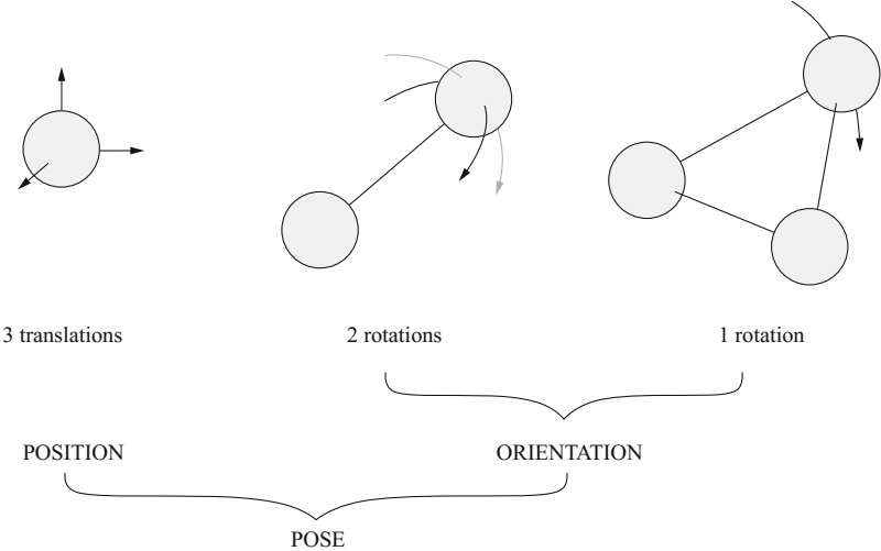
Fig. 1.4 Degrees of freedom of a rigid body
