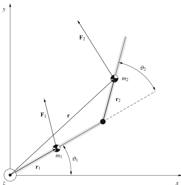
Fig. 5.12 Planar robot manipulator approximated by point masses m_1 and m_2
