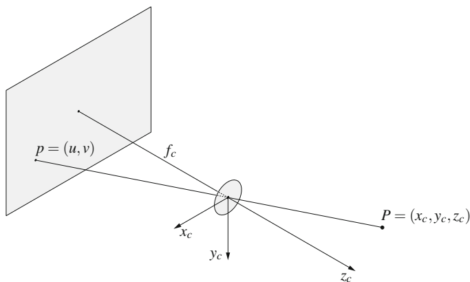
Fig. 8.1 Perspective projection
