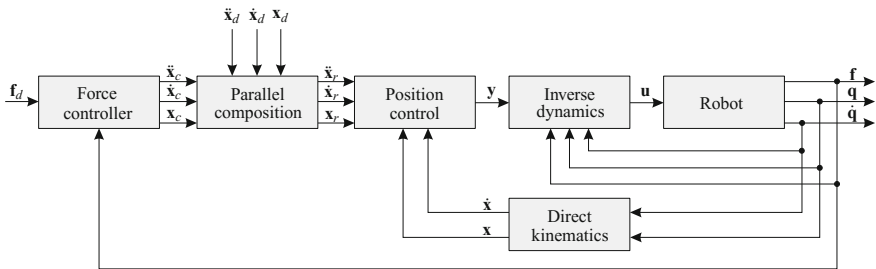
Fig. 10.16 Direct force control in the external coordinates
