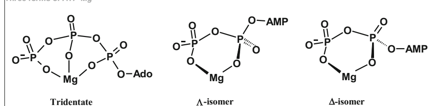
Three forms of ATP-Mg
