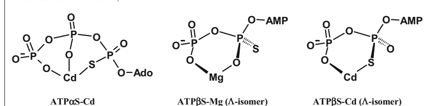
Thio-substituted ATP-Me complexes
