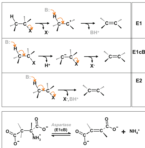
Fig. 29.9 Three possible elimination reaction mechanisms. While the E1 reaction goes through a carbocation intermediate, the E1cB mechanism involves a carbanion intermediate. In the E2 mechanism, breaking of C–H and C–X bonds is simultaneous. Aspartase reaction (shown below) follows E1cB mechanism where the C–N bond breaks to eliminate ammonium
