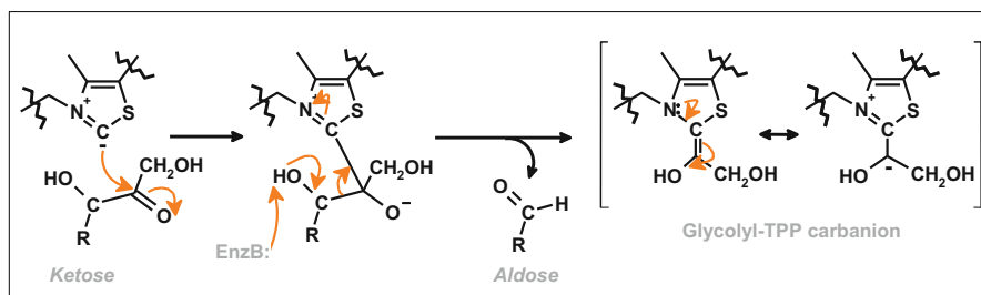
Fig. 34.9 Transketolase mechanism involving a glycolyl-TPP carbanion. Reaction for the synthesis of sedoheptulose-7-P is shown, for example. Glyceraldehyde-3-P is released from ribulose-5-P, while the glycolyl group is retained on the TPP. In a reversal of these steps, ribose-5-P accepts the glycolyl group to form sedoheptulose-7-P
