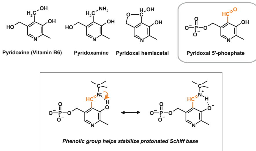
Fig. 35.5 Structures of pyridoxine, pyridoxamine, pyridoxal hemiacetal, and pyridoxal phosphate. The aldehyde group is masked in free pyridoxal as it forms hemiacetal. Phosphorylation of the -\text{CH}_2\text{OH} group ensures that the PLP aldehyde does not form a hemiacetal and is free to react with amino groups. The phenolic -\text{OH} on the pyridine ring is suitably positioned to stabilize the protonated PLP Schiff base (right, box below) during reaction. The positively charged N atom tends to withdraw electrons from \text{C}_\alpha of the amino acid – thereby weakening its binding to -\text{H} , -\text{R} , and -\text{COO}^- .
