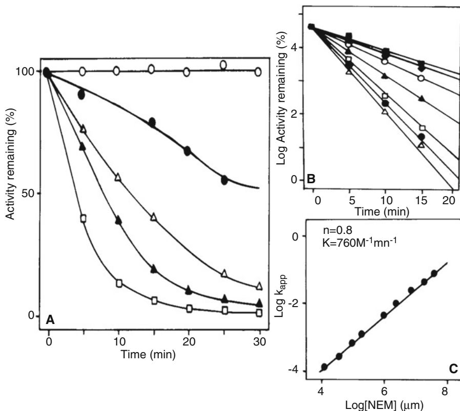
Fig. 21.1 N-Ethylmaleimide inactivation of glutamine synthetase. The time course of inactivation (A), semilog plot of the same data (B), and a replot \log k_{\text{obs}} \rightarrow \log [I] (C) are shown
