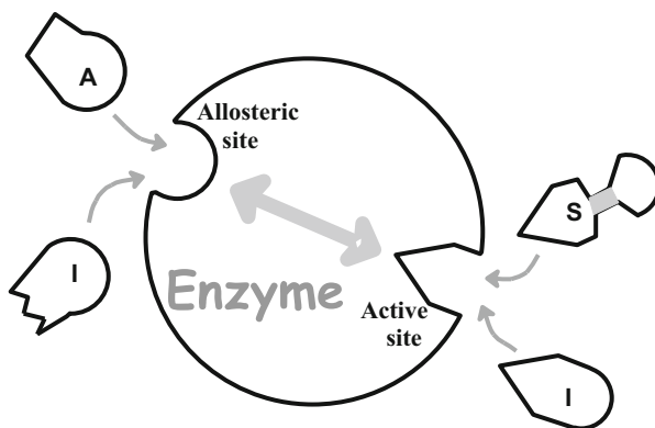
Fig. 5.2 Schematic of an enzyme showing different ligand binding sites. Possible binding to substrate (S), activator (A), and inhibitor (I) is shown. The susceptible bond in the substrate is shown in gray
