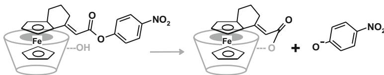
Fig. 39.3 A \beta -cyclodextrin mimic of chymotrypsin displaying catalysis of p -nitrophenyl ester hydrolysis. The cyclodextrin cavity binds the hydrophobic ferrocene core of the ester substrate
