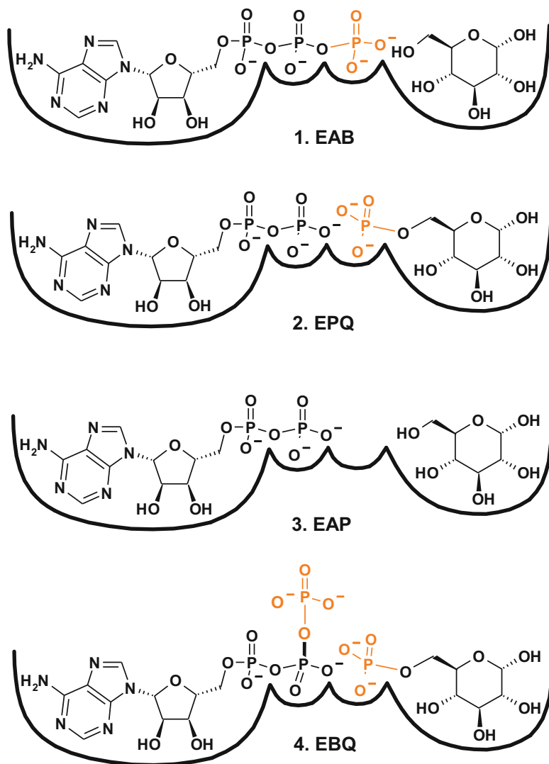
Fig. 28.3 Different ternary complexes possible with the enzyme in a kinase mechanism. The scheme is for hexokinase with glucose and is simplified by not showing \text{Mg}^{2+} in \text{Mg-ATP} . The four complexes are (1) EAB ( \text{E.Mg-ATP.glucose} ), (2) EPQ ( \text{E.Mg-ADP.glucose 6-phosphate} ), (3) EAP ( \text{E.Mg-ADP.glucose} ), and (4) EBQ ( \text{E.Mg-ATP.glucose 6-phosphate} )
