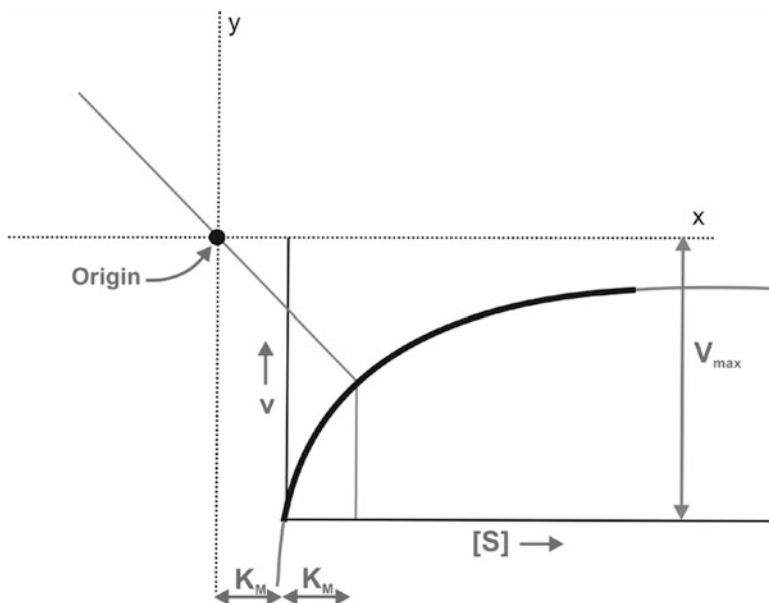
Fig. 15.3 The v \rightarrow [S] curve described by the Michaelis–Menten equation is part of a rectangular hyperbola. The highlighted short arc (dark line) is the actual region where experimental observations for an enzyme are physically possible. The two limbs of this rectangular hyperbola form asymptotes of an infinite curve as shown. This makes direct estimation of both K_M and V_{\max} values difficult
