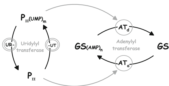
Fig. 37.10 The covalent regulation of E. coli glutamine synthetase. The uridylylation cycle and adenylation cycle are linked through the regulatory protein \text{P}_{\text{II}} . Glutamine is an activator of UR activity, while 2-oxoglutarate activates UT. The \text{P}_{\text{II}} protein activates \text{AT}_a , while \text{P}_{\text{II}}\text{-UMP} activates \text{AT}_d . Ultimately, \text{AT}_a and \text{AT}_d are, respectively, responsible for the adenylation and the deadenylation of glutamine synthetase. \text{AT}_a transfers AMP from ATP to form one adenylyl-O-tyrosyl bond per each subunit of the dodecameric glutamine synthetase (where n = 1\text{--}12 ). Covalent modification by UT similarly involves the transfer of UMP from UTP to \text{P}_{\text{II}} (where n = 1\text{--}3 )
