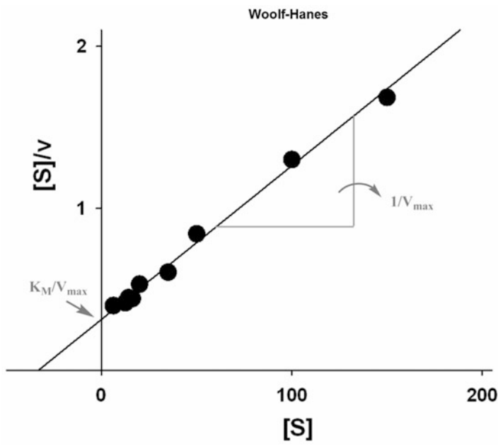
Fig. 17.7 The Woolf–Hanes single-reciprocal plot. Arginase data from Table 17.3 was graphed as [S]/v \rightarrow [S] plot
