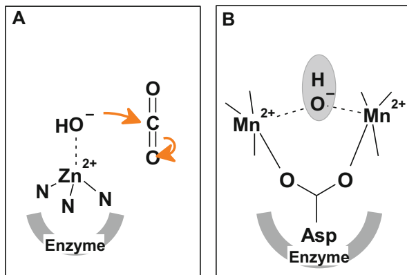
Fig. 6.7 Metal ions enhance the nucleophilicity of water during catalysis.
