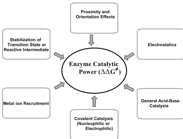
Fig. 6.1 Various features that enzymes use to achieve reaction rate acceleration
