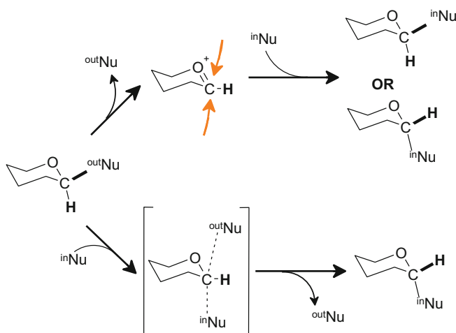
Fig. 27.5 Mechanism of glycosyl transfer: The two possible paths for this reaction are a stepwise mechanism (via an oxycarbonium; upper route) or a \text{S}_{\text{N}}2 mechanism (second-order nucleophilic substitution; lower route). The atoms where \alpha -secondary KIE is measured are in bold
