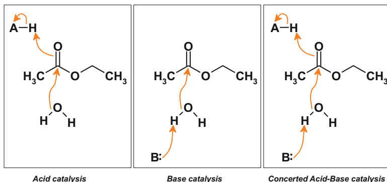
Fig. 30.5 Acid–base-catalyzed hydrolysis of ethyl acetate. Ester hydrolysis may be facilitated by the acid AH (acid catalysis), the base B: (base catalysis), or both (in concert). In water, when \text{AH} = \text{H}^+ , it is specific acid catalysis and when \text{B:} = \text{OH}^- , it is specific base catalysis. Concerted acid–base catalysis involves simultaneous presence and action of a general acid (AH) and a general base (B:). Such an arrangement of groups is best provided at enzyme active sites shielded from the bulk aqueous medium
