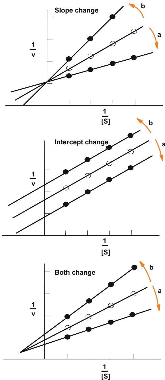
Fig. 18.1 Possible changes in the slope and intercept of double-reciprocal plots.
