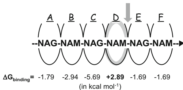
Fig. 7.1 Substrate binding at the lysozyme active site.
