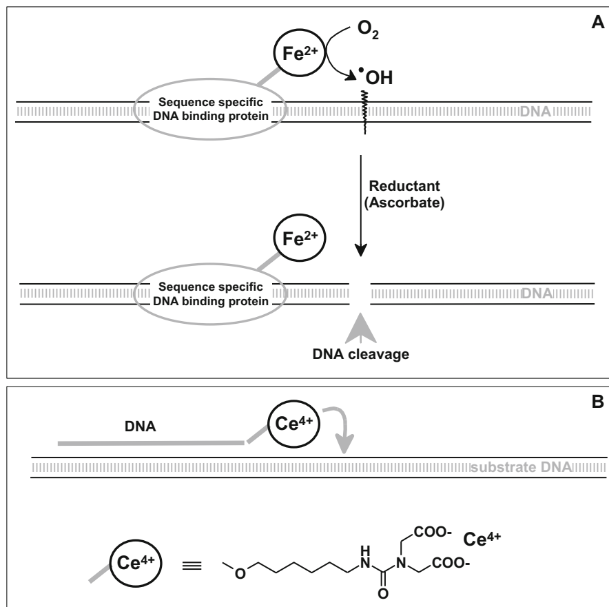
Fig. 39.2 Construction of artificial restriction enzymes (A) Fenton chemistry of EDTA-Fe(II) with oxygen generates hydroxyl ( HO^\bullet ) radicals for local DNA cleavage. Specificity is provided by using a unique sequence-recognizing moiety (e.g., trp or lac repressor or catabolite activator protein of E. coli ). (B) A restriction enzyme construct of Ce^{4+} complex of iminodiacetate. This Ce^{4+} nuclease is juxtaposed to the specified DNA sequence for cleavage by an oligonucleotide sequence-recognizing moiety
