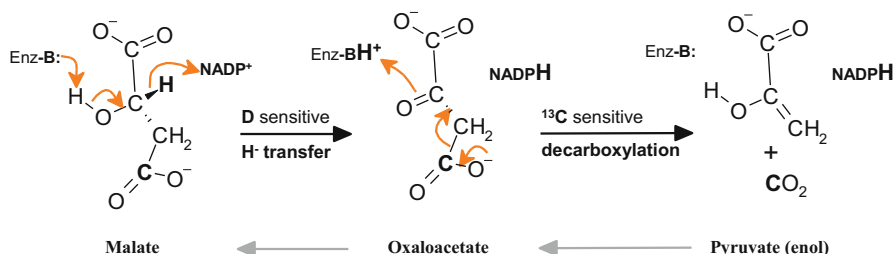
Fig. 27.4 Deuterium- and ^{13}\text{C} -sensitive steps in the reaction mechanism of malic enzyme. The dotted arrows indicate the sequence of events in the direction of reverse reaction
