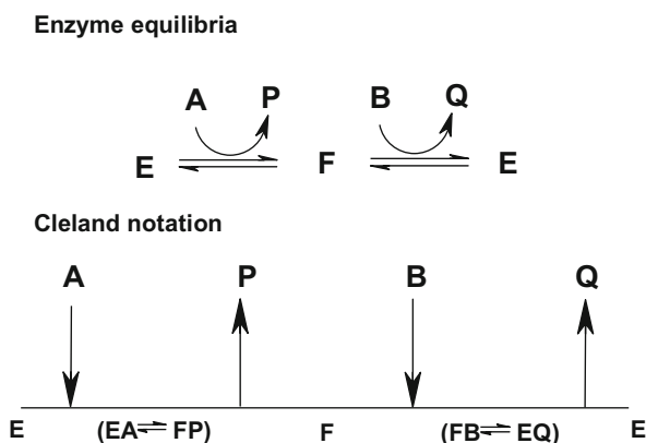
Fig. 19.3 Equilibria representing a bi-reactant ping-pong mechanism
