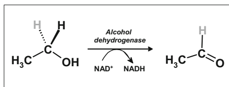
Fig. 29.7 Stereochemistry of alcohol dehydrogenase reaction. Only the proR -hydrogen of ethanol is selectively removed by the enzyme. The C-1 of ethanol is an example of prochiral carbon with abc arrangement of groups around it. The proR -hydrogen is shown in black and proS -hydrogen is in gray
