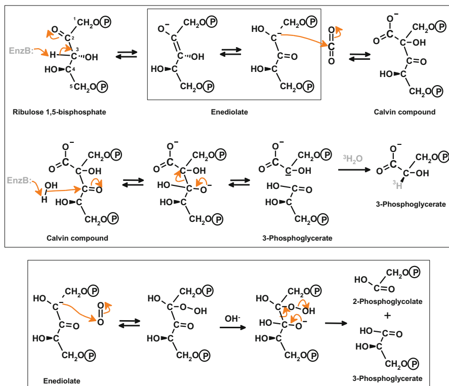
Fig. 34.3 Carboxylation reaction mechanism of ribulose-1,5-bisphosphate carboxylase-oxygenase. The bottom panel shows the oxygenase reaction catalyzed by the same enzyme. The carbon originating from \text{CO}_2 is in bold
