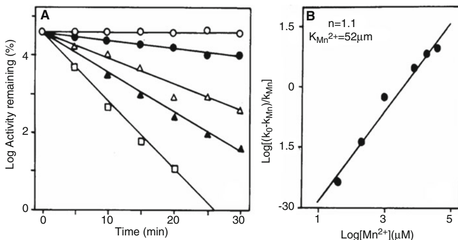
Fig. 21.2 Protection afforded by Mn^{2+} ions during N-ethylmaleimide inactivation of glutamine synthetase. Pseudo-first-order plots (A) and the corresponding replot (B) of \log[(k_0 - k_{Mn})/k_{Mn}] \rightarrow \log[Mn^{2+}] are shown
