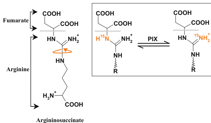
Fig. 25.2 Positional isotope exchange (PIX) in argininosuccinate lyase reaction. Gray line shows the C-N bond cleaved by the enzyme, and the cyclic arrow indicates a free rotation around that bond at the enzyme active site
