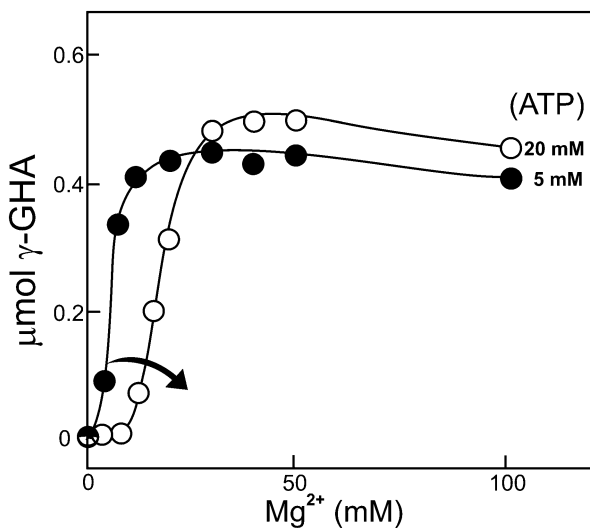
Fig. 32.3 \text{Mg}^{2+} saturation profile of glutamine synthetase
