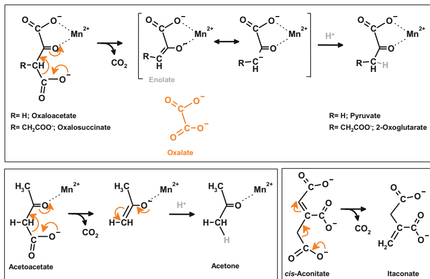
Fig. 34.5 Decarboxylation of \beta -keto acids. Among the carboxylate groups, the carboxylate that has a suitably positioned \beta -keto moiety is lost as CO 2 . Mn 2+ functions to accept the developing negative charge. Proposed decarboxylation of cis -aconitate by exploiting appropriately located double bond is also shown
