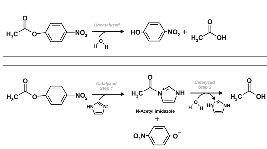
Fig. 31.1 Imidazole-catalyzed hydrolysis of 4-nitrophenyl acetate. Both acetylation of imidazole (Step 1) and hydrolysis of acetyl imidazole (Step 2) are faster than the direct interaction of 4-nitrophenyl acetate with water (uncatalyzed reaction). Imidazole is a true nucleophilic catalyst since it is recovered intact after the reaction and acetyl imidazole forms during catalysis
