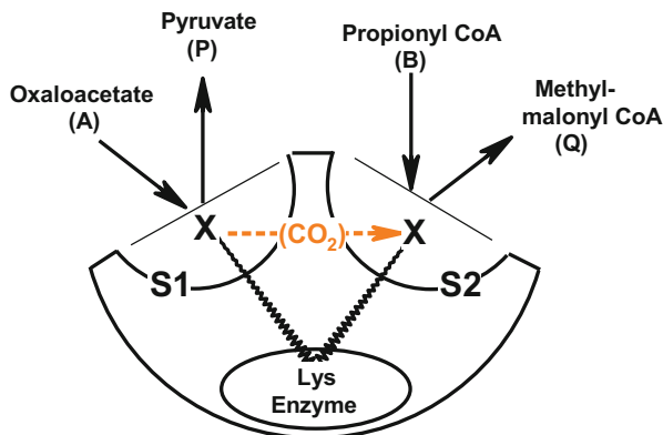
Fig. 28.5 Schematic representation of the transcarboxylase reaction. Oxaloacetate (A) and pyruvate (P) interact with site S1 while the thioester pair (propionyl CoA and methylmalonyl CoA, shown as B and Q, respectively) interacts at the S2 site. The swinging arm with biotin (X) shuttles the carboxyl group from S1 to S2
