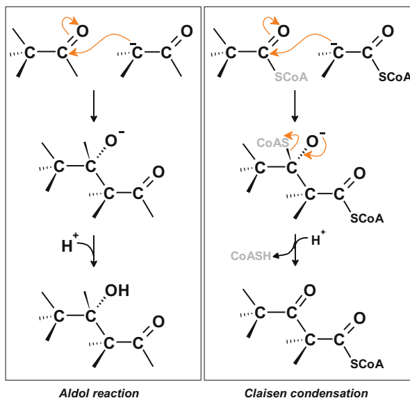
Fig. 29.10 Biochemically important carbon–carbon bond-forming reactions.
