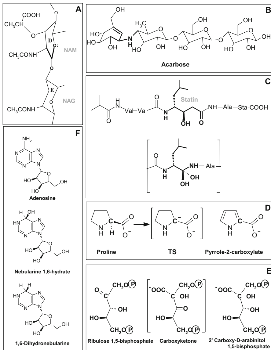
Fig. 6.9 Transition state binding and stabilization. (A) Half-chair conformation of the NAM sugar bound to lysozyme active site; (B) acarbose, \alpha -glucosidase inhibitor; (C) structure of statin found in pepstatin and the corresponding enzyme-bound tetrahedral intermediate; (D) the planar TS of proline racemase and pyrrole 2-carboxylate; (E) the carboxyketone intermediate of RubisCO and its inhibitor analog 2'-carboxy-D-arabinitol 1,5-bisphosphate; (F) nebularine 1,6-hydrate is a potent inhibitor of adenosine deaminase because of the -OH group on the tetrahedral C-6 of purine
