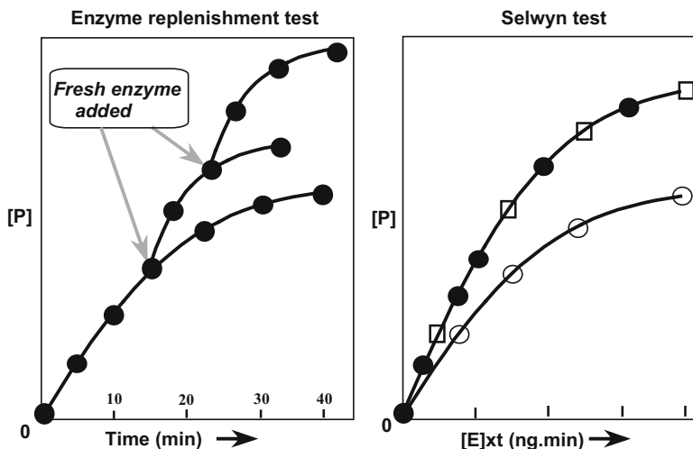
Fig. 13.1 Enzyme inactivation during assay. This may be tested by fresh addition of enzyme (left panel) and by Selwyn test (right panel). The curves for two different enzyme concentrations (● and □) superimpose when there is no inactivation. With inactivation however, the curve for lower enzyme concentration (○) is distinct and falls off much faster
