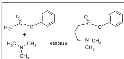
Fig. 6.2 Organic model reactions exemplifying the proximity and orientation effects that lead to rate accelerations. Hydrolysis of phenyl esters by carboxylate (A), tertiary amine (B), and imidazole (C) is shown
