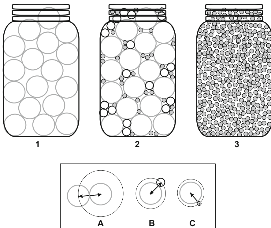
Fig. 38.2 Visualization of crowding effects. A glass jar can be filled by large- (Jar 1), small- (Jar 3), or medium-sized spheres. Jar 3 cannot further accommodate any of these spheres. However, Jar 1 can still accommodate medium-/small-sized spheres in between (Jar 2). This is because large spheres exclude more volume from around them. Similarly, a macromolecule in solution will exclude others from its neighborhood. The position of each molecule is specified completely by the position of its center. The closest any two molecules (assumed as spheres; box below) can approach is a distance equal to the sum of their radii. Around each molecule is a spherical volume from which the centers of all others are excluded. For instance, the volume around a macromolecule from which the center of another similar molecule is excluded is a sphere of radius twice (eight times the volume) that of a single molecule (case A in the box below)
