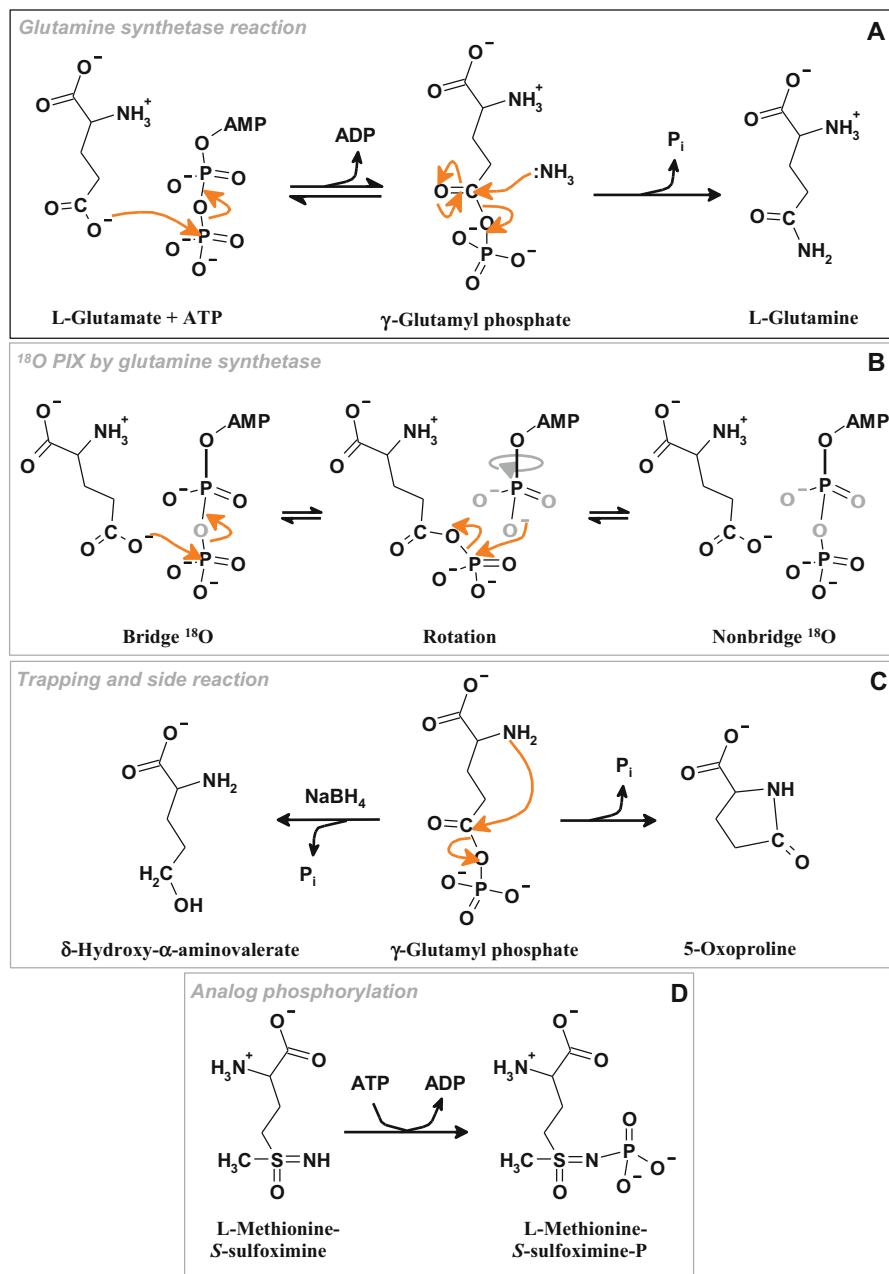
Fig. 31.5 Glutamine synthetase catalysis proceeds via \gamma -glutamyl phosphate as the obligate covalent reaction intermediate. (A). Glutamine synthetase reaction. (B). Scrambling of 18 O-label evidenced by PIX. (C). Trapping \gamma -glutamyl phosphate by NaBH 4 reduction and 5-oxoproline forming side reaction. (D) Phosphorylation of L-methionine-S-sulfoximine
