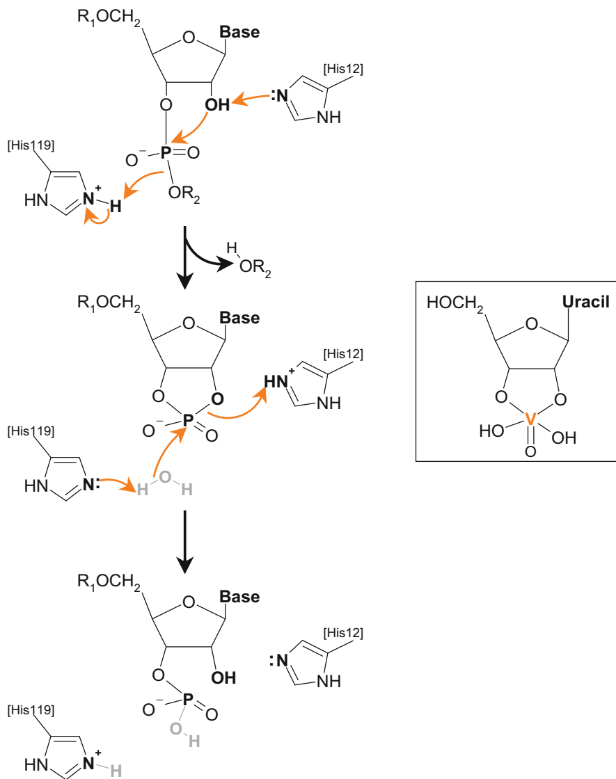
Fig. 36.9 Reaction mechanism of RNase A. His-12 imidazole group (base) abstracts the proton from 2'-OH, while His-119 imidazole group (acid) protonates the leaving group \text{OR}_2 (the 3' portion of the RNA substrate). The 2',3'-cyclic phosphate is opened up by water where the roles of His-12 and His-119 are reversed. The enzyme specificity controls this step so that only the 3'-phosphate results. Structure of uridine vanadate (a potent inhibitor) is shown in the box
