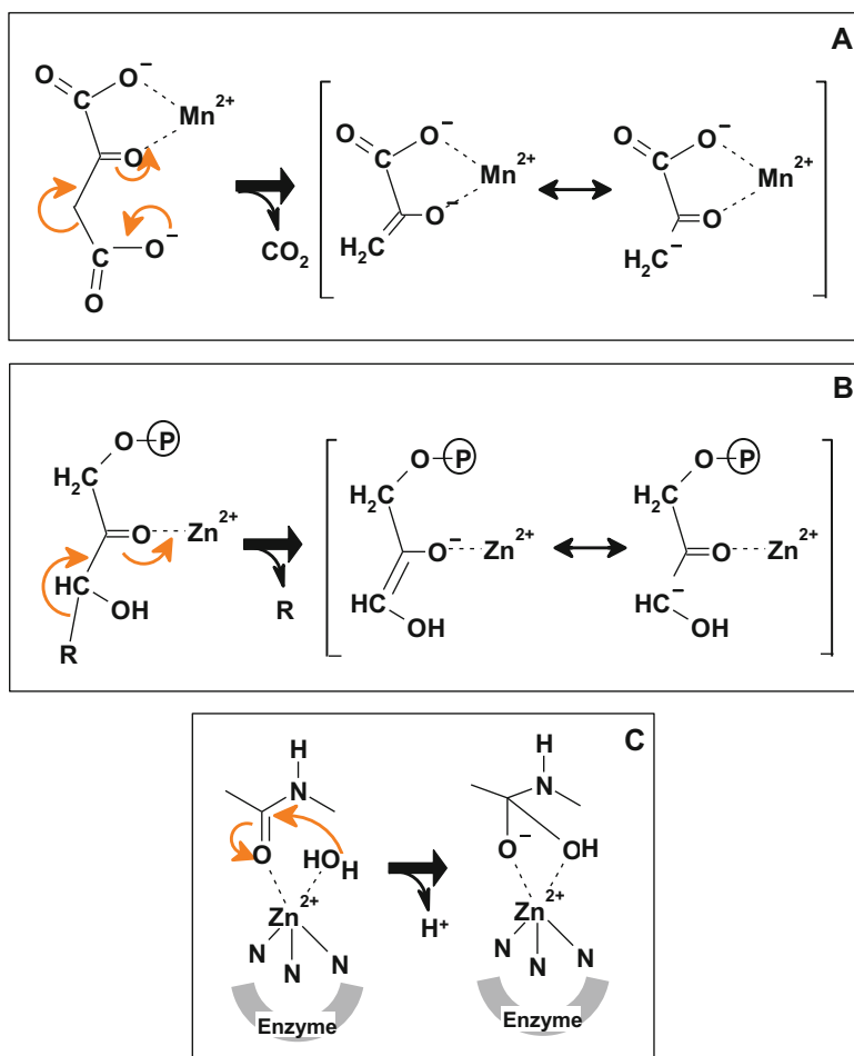
Fig. 6.6 Metal ions involved in charge stabilization during catalysis. (A) Oxaloacetate decarboxylase - \text{Mn}^{2+} ; (B) class II aldolase - \text{Zn}^{2+} ; (C) carboxypeptidase A - \text{Zn}^{2+}
