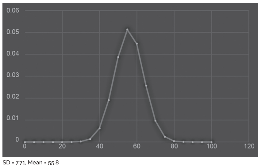
Figure A.6 Normal Distribution and Standard Deviation Analysis.
