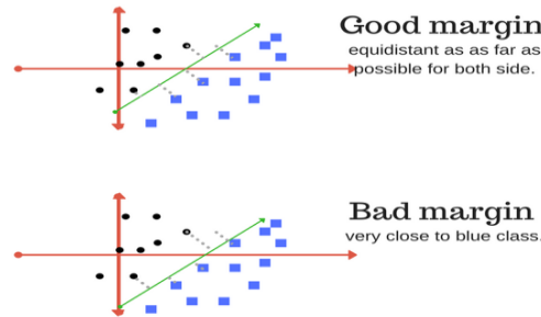
Figure 4. Hyperplane [20]
