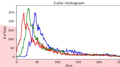
Figure 3. Color Histogram
