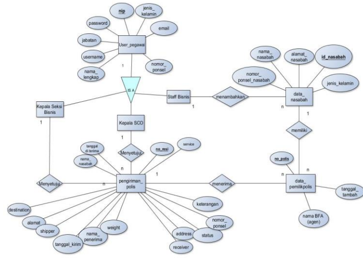
Gambar 4.5 Entity Relation Diagram (ERD)
