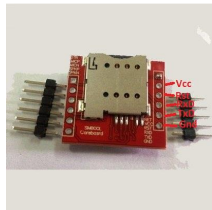
Gambar 5 SIM800I
