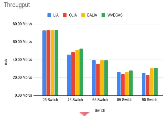
Gambar 7. Grafik Throughput
