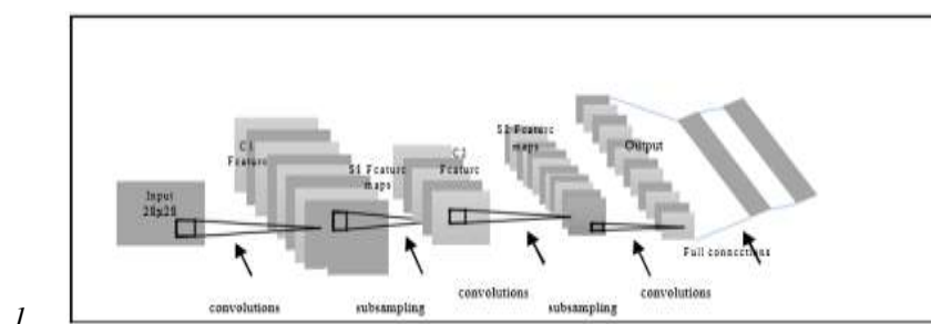
2. Gambar 2. 1 Struktur Convolutional Neural Network
