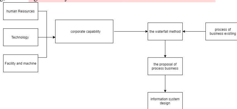
Figure 2 Conceptual Model
