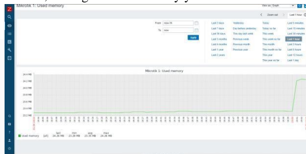
Gambar 4.5 (a) Used Memory
