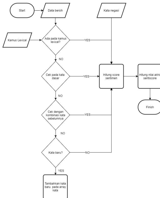
Gambar 3 Flowchart Perhitungan Sentimen Score
