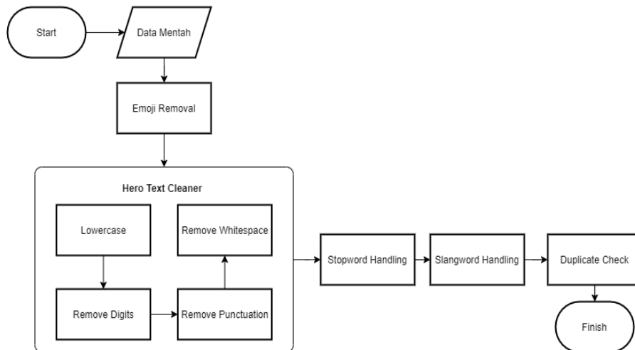
Gambar 2. Flowchart Preprocessing Sistem
