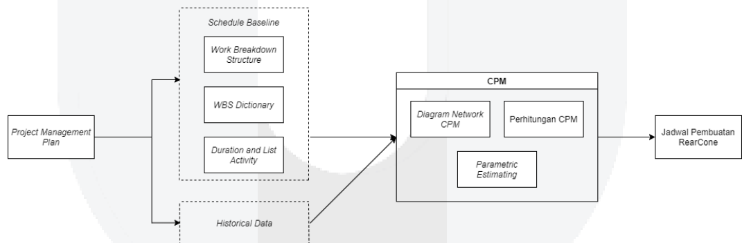
Gambar 3.1 Model Konseptual
