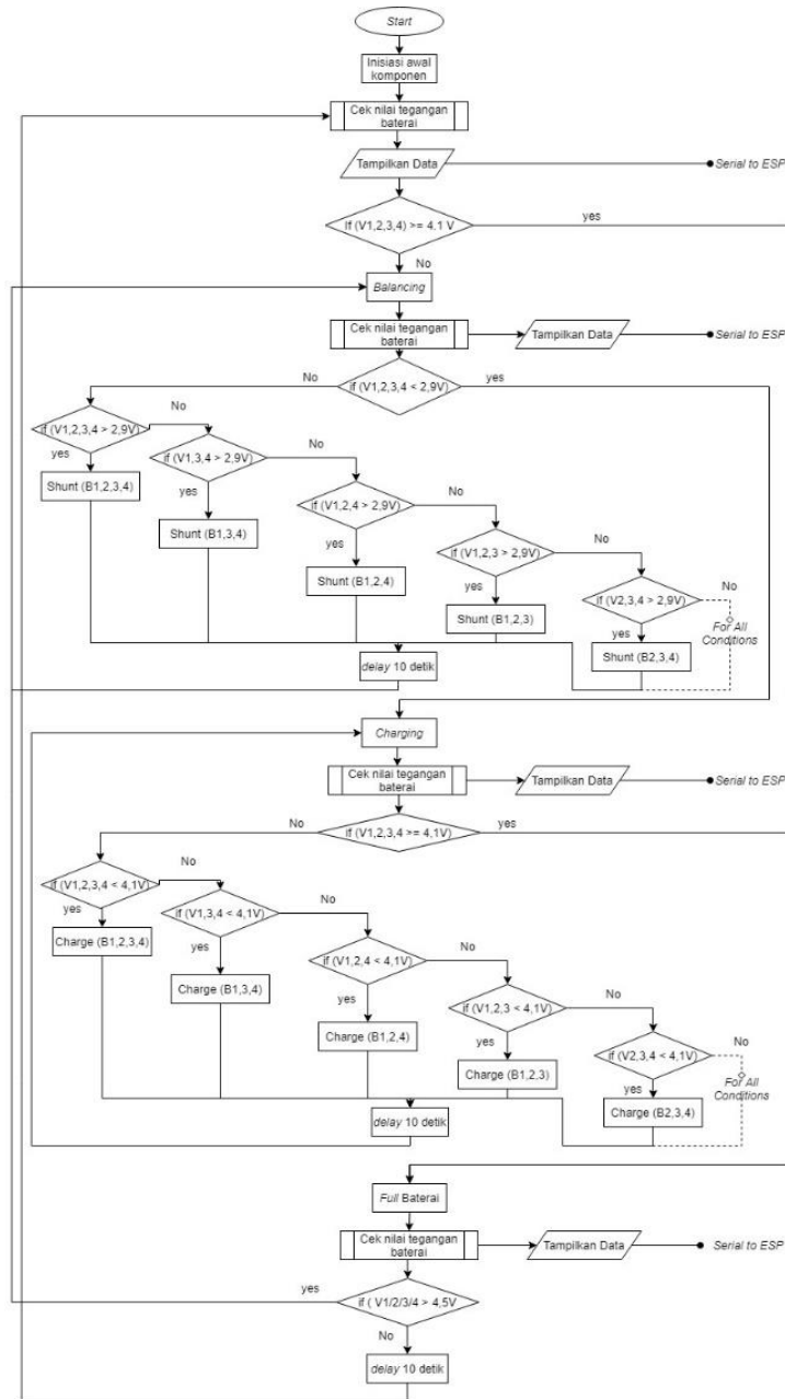
Gambar 3. Flowchart Arduino
