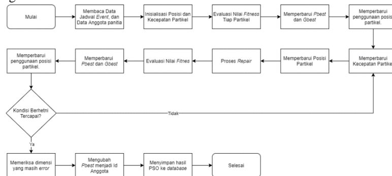
Gambar 3. Flow Chart Proses PSO
