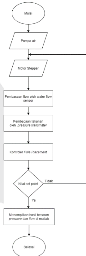
Gambar 6. Diagram alir
