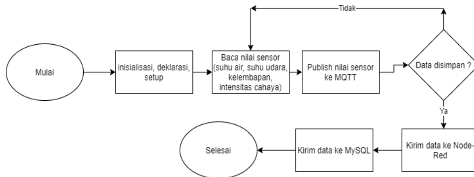
Figure 1. System Flowchart
