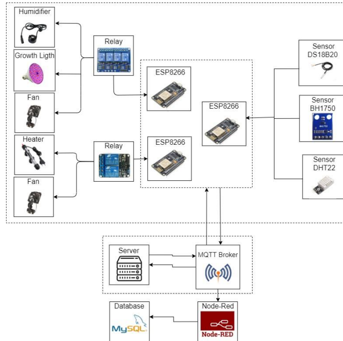
Figure 2. Block Diagram
