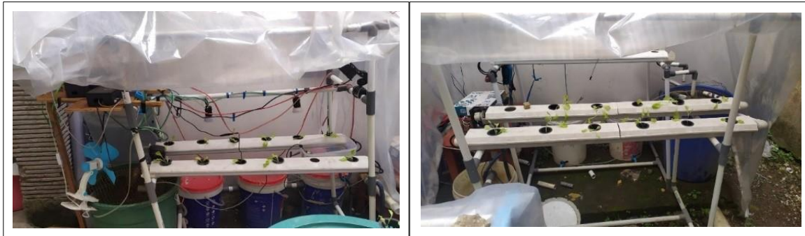
Figure 3. Aquaponics with IoT (left) & Aquaponics Conventional (right)
