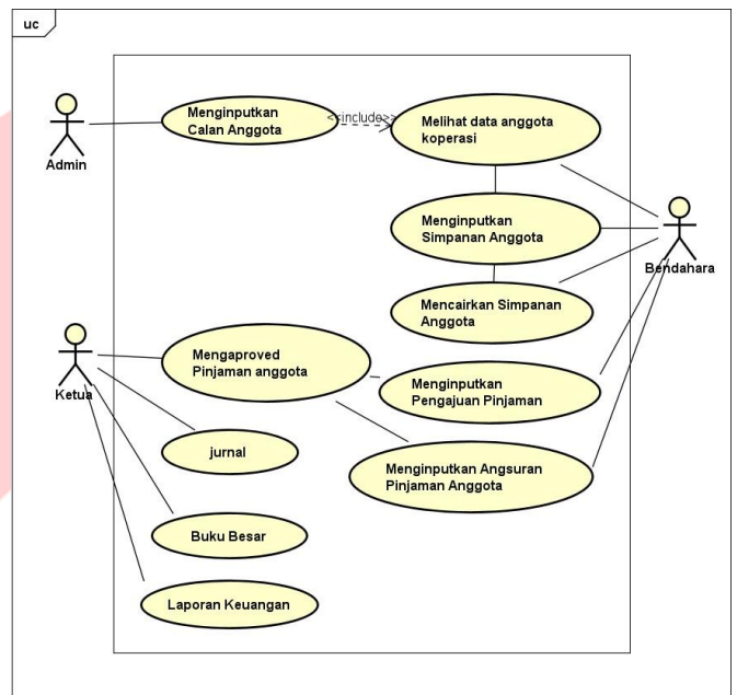
Gambar 1 Usecase Diagram
