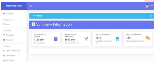
Gambar 6 Interface Dashboard
