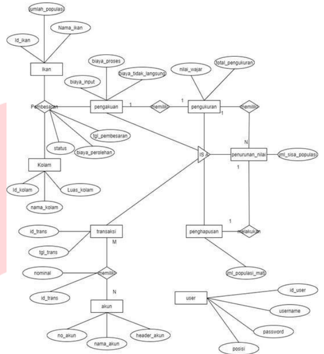
Gambar 3 Entity Relationship Diagram
