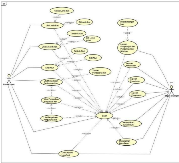
Gambar 1 Usecase Diagram
