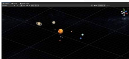
Gambar 43 Tata Surya
