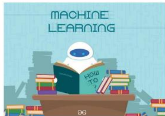
Gambar 2 Machine Learning
