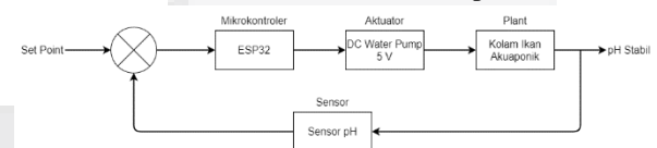
GAMBAR 3 Diagram Blok Sistem Kendali
