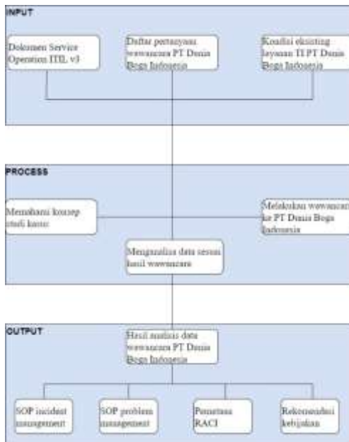
GAMBAR 3.1 Model Konseptual
