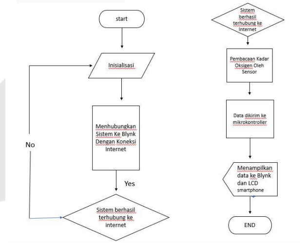
Gambar 4 Flowchart
