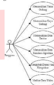
Gambar 3 Use Case diagram.
