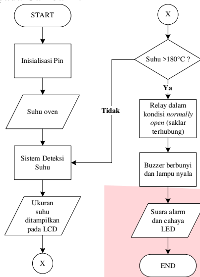
GAMBAR 4. FLOWCHART DIAGRAM SISTEM KERJA SENSOR
