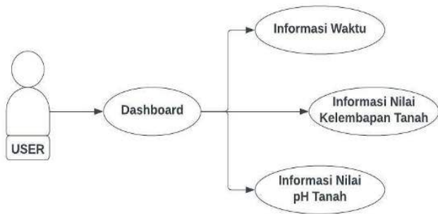
GAMBAR 3.5 USE CASE
