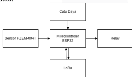
GAMBAR 3 BLOK DIAGRAM PANEL SISTEM
