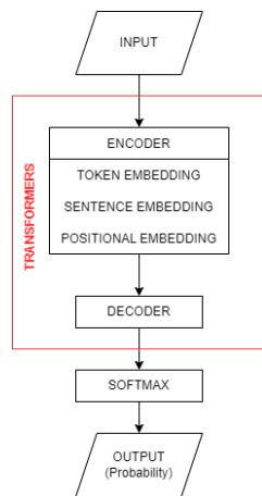
GAMBAR 5 FLOWCHART ALGORITMA BERT
