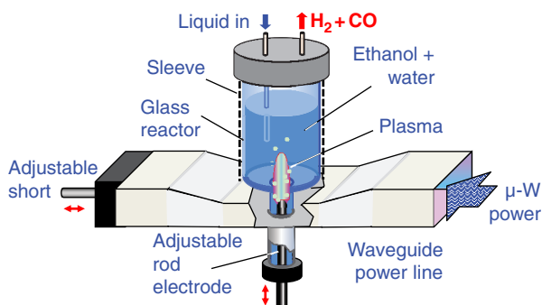
Figure 6.4 Illustration of the experimental system for production of hydrogen-rich gas.
