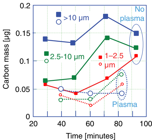
Figure 5.25 Plasma removal of the particulate matter from the diesel genset. The graph shows differences before and after plasma treatment according to particle size.
