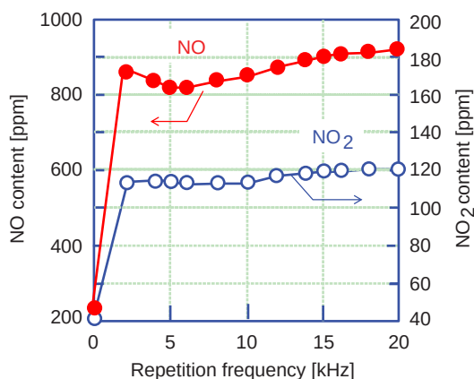
Figure 5.26 Generation of NO and NO 2 in the microwave air plasma-treated diesel exhaust as a function of the repetition frequency of the microwave power pulses.
