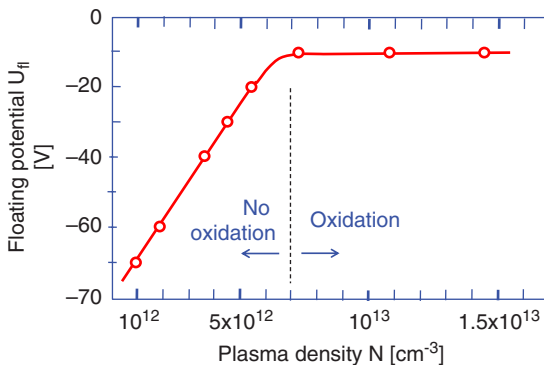
Figure 4.16 The floating potential vs the plasma density. Parameters: P \leq 3 kW (3 ms, 50 Hz), p_{O_2} = 0.4 Pa, B = 1.43 B_{ce} .
