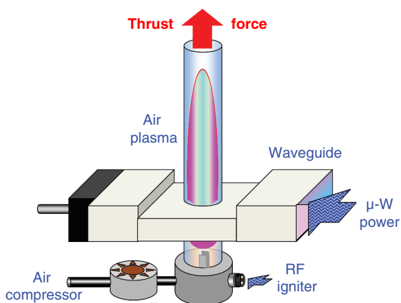
Figure 6.3 An illustration of the experimental system for testing the thrust force of the atmospheric microwave air plasma.
