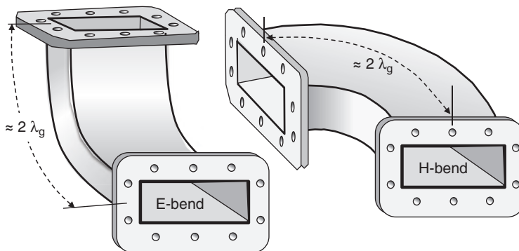
Figure 1.15 Illustrations of typical 90^\circ waveguide bends in the E direction and H direction.
