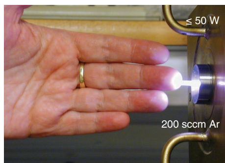
Figure 5.6 The effect of the pulsed DC hollow cathode (0.5 \mu s, 250 kHz, 50 W) on the power transferred by the plasma plume in the H-HEAD plasma source. The nozzle became hot.
