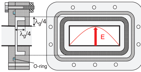
Figure 1.16 An illustration of a choke-type flange connection between waveguide components.
