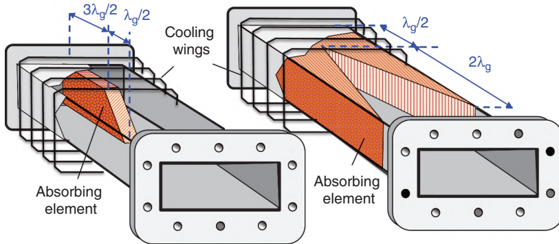
Figure 1.20 Examples of waveguide attenuators. Air cooling wings can be replaced by a barrel with cooling water.
