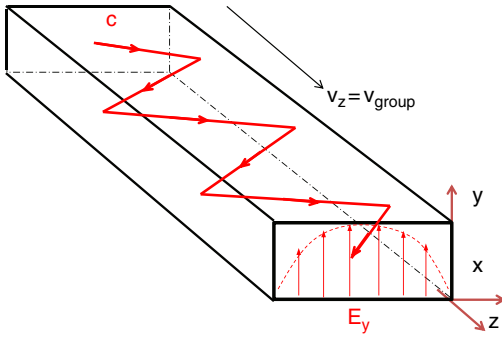
Figure 1.4 Schematic description of the reflection of the propagating TE_{10} wave in a lossless waveguide. Value ( v_{group} ) is the velocity of propagating the wave power.
