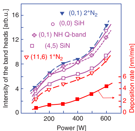
Figure 4.29 Comparison of the power functions of the intensities of the most intense band heads and the growth rate of the silicon nitride. Total pressure p_{\text{TOT}} = 80 Pa (0.6 Torr). Substrate temperature T_{\text{sub}} = 300^\circ\text{C} .
