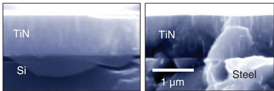
Figure 4.55 The scanning electron microscope (SEM) image of the fracture cross-sections of the 1 µm thick TiN films on silicon and on stainless steel substrate.
