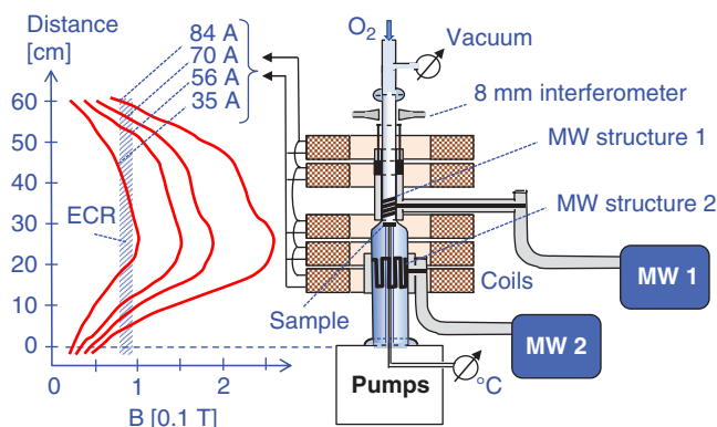
Figure 4.13 Schematic of the experimental system for oxidation of silicon samples in a magnetoactive microwave plasma. Diameters of the quartz discharge tube were 33 mm (upper part) and 80 mm (lower part). Maximum induction in the axis of the tube increased to 4 B_{CE} .
