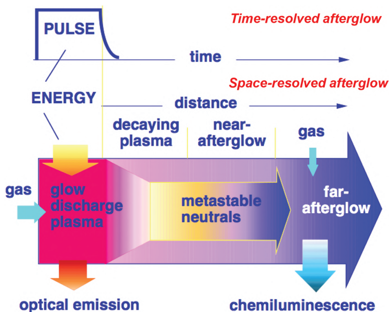
Figure 3.5 Time-resolved and space-resolved afterglows. Certain gases can be excited by long-lived metastable particles from plasma. Recombination processes can produce visible light (chemiluminescence), see also Ref. [3.13].
