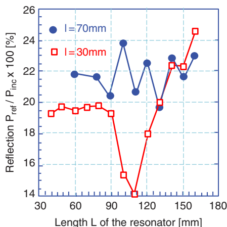
Figure 4.37 Adjusting the reactor length L to resonance at two different lengths l of the antenna. Antenna gas was 300 sccm H_2 + 3 sccm CH_4 . Auxiliary gas was 100 sccm Ar + 1 sccm O_2 . The incident power was P_{inc} = 400 W, the gas pressure in the reactor was p_{TOT} = 5 Torr.
