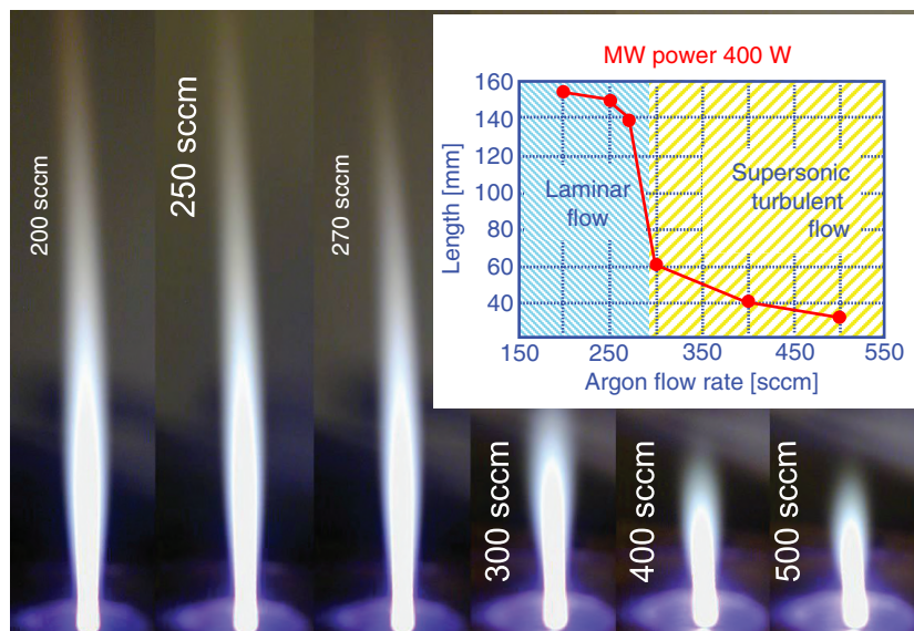
Figure 5.9 Dependency of the argon plasma plume length at 400 W power in the H-HEAD source on the argon flow rate.
