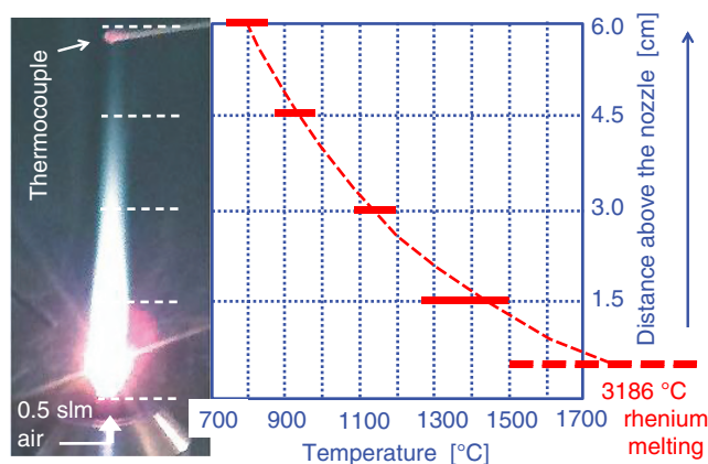
Figure 5.33 The temperature of the microwave air plasma jet at different distances from the nozzle on the microwave antenna. The temperature near to the nozzle was close to the melting point of rhenium cartridge of the thermocouple (3186°C).
