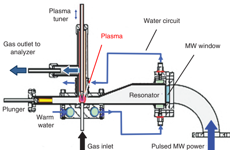
Figure 5.23 The system with pulsed power of 2.4 GHz, up to 1 kW in 1–20 kHz pulses (duty cycle 1) for testing of removal particulate matter from 2 kW diesel genset exhaust.
