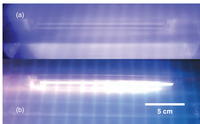
Figure 4.53 View on the argon plasma at 6 mTorr (0.8 Pa) pressure in the HYP source through the window shielded by a metallic shielding net. (a) The ECR plasma at 1 kW. (b) The ECR plasma with the RF hollow cathode plasma generated by the M-M source at 1 kW power.
