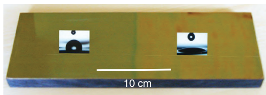
Figure 5.12 An increased hydrophobicity on the right part of the carbon fiber sample after several scans by the H-HEAD plasma.
