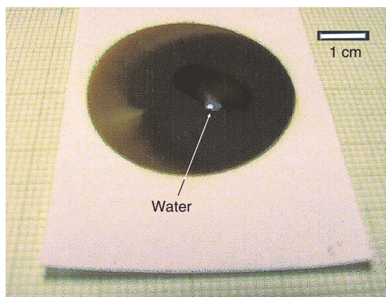
Figure 4.50 A filter-paper substrate coated 10 min by the \text{CN}_x film on a 30 mm diameter area was capable of keeping the water droplet.
