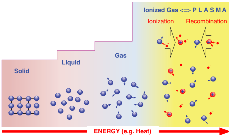
Figure 2.1 Simple schematic description of the phases of matter and the formation of the plasma state.
