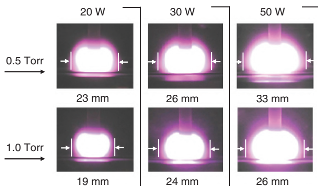
Figure 4.40 Photographs of the ball plasma generated in N_2 + C_2H_2 gas at different microwave powers for two reactor pressures. Diameter of the plasma ball depends on both parameters.
