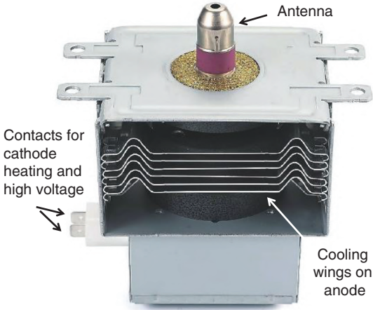
Figure 1.28 Shapes of typical air-cooled microwave magnetron tubes used in microwave ovens.
