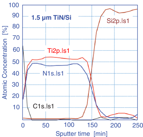
Figure 4.56 The ESCA depth profile in the 1.5 µm thick TiN film deposited 10 min by the reactive PVD on Si substrate in the HYP source. The process parameters: 6 mTorr, 70 sccm (Ar + 10% N 2 ), RF power 3 kW, µW power 1.2 kW.
