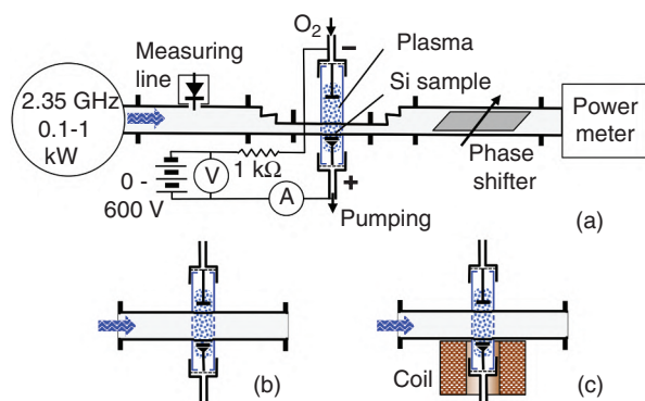
Figure 4.4 Schematic of the waveguide system for microwave generation of oxygen plasma in 40 mm outer diameter tube (a). A discharge section in the untapered waveguide (b). An arrangement with magnetic coil for study of motions of charged particles (c).
