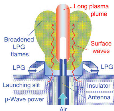
Figure 5.32 Schematic representation of experimental arrangement for testing the effects of microwave antenna plasma on the LPG flames.
