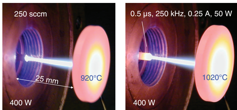
Figure 5.6 The effect of the pulsed DC hollow cathode (0.5 \mu s, 250 kHz, 50 W) on the power transferred by the plasma plume in the H-HEAD plasma source. The nozzle became hot.
