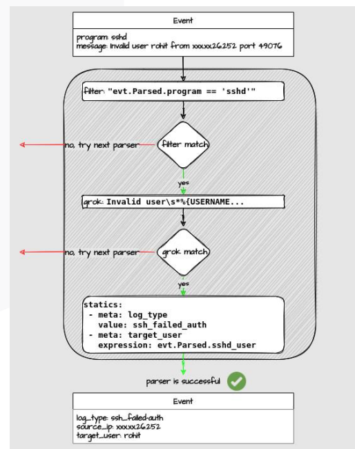
GAMBAR 1 PARSERS WORKFLOW
