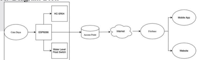
GAMBAR 3 DIAGRAM BLOK
