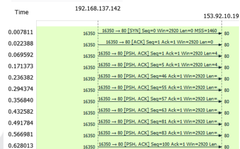
GAMBAR 4.2 FLOW GRAPH
