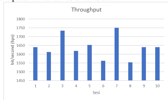
GAMBAR 4.7 GRAFIK THROUGHPUT
