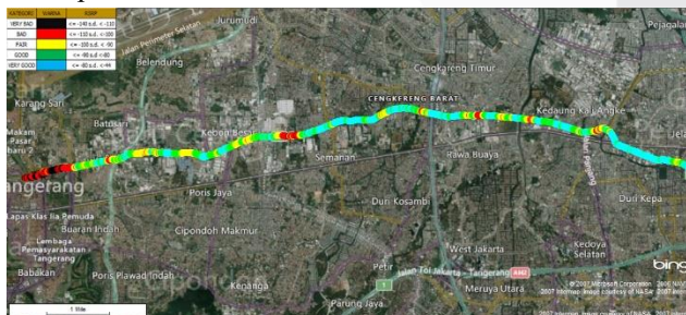
GAMBAR III HASIL RSRP DRIVE TEST I
