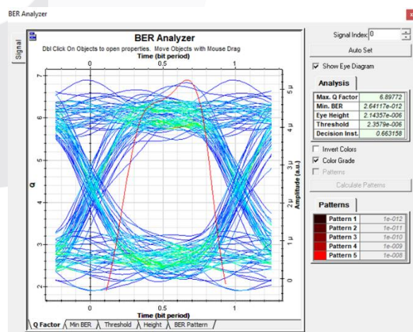
Gambar 8. BER-analyzer Simulasi Backhaul
