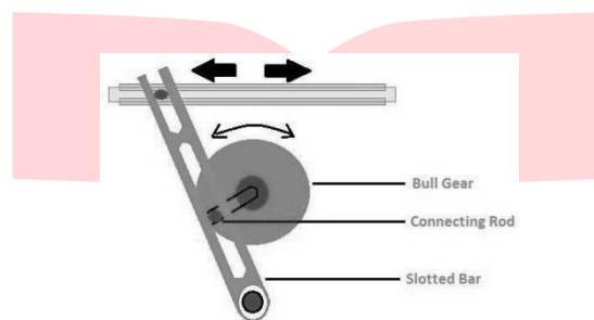
Gambar 5 Mekanisme quick-return Sumber: mechanicbasics.com
