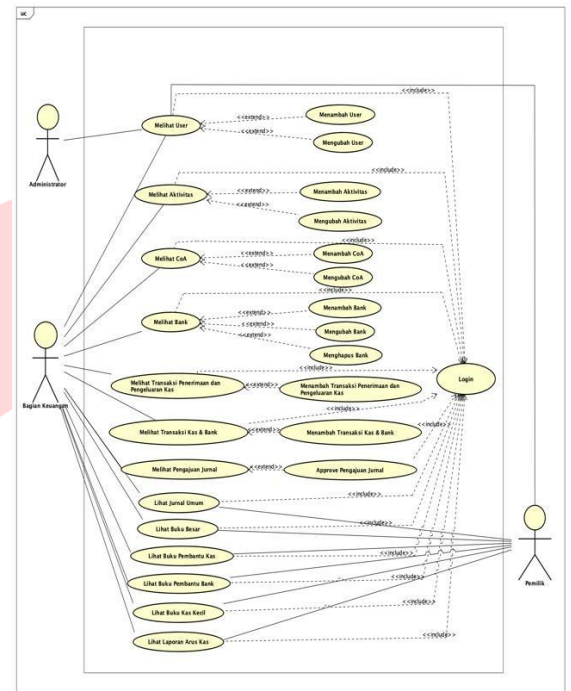
GAMBAR 1- 4 Usecase Diagram
