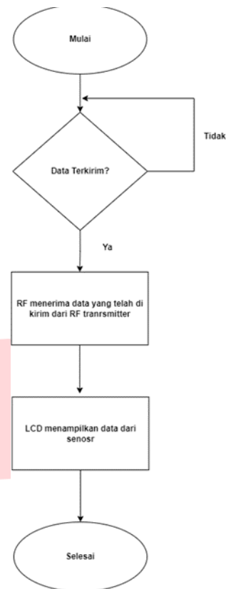
GAMBAR 3 FLOWCHART RECEIVER
