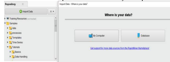
GAMBAR 4. 2 IMPORT DATA
