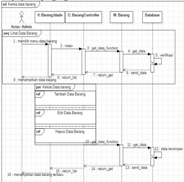
GAMBAR 11 (SEQUENCE DIAGRAM)
