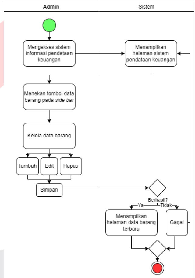
GAMBAR 10 (ACTIVITY DIAGRAM)
