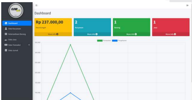
GAMBAR 13 (TAMPILAN DASHBOARD)
