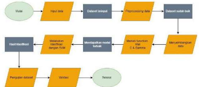
GAMBAR 3 (PERANCANGAN METODE SUPPORT VECTOR MACHINE)
