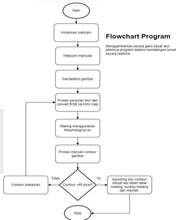
GAMBAR 3 FLOWCHART
