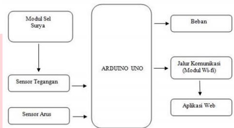
Gambar 3.1 Blok Diagram
