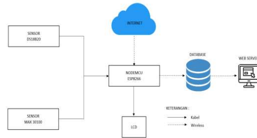
Gambar 3.1 Blok Diagram
