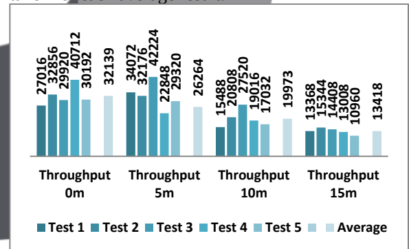
Figure 4.13. Average throughput per session results.
