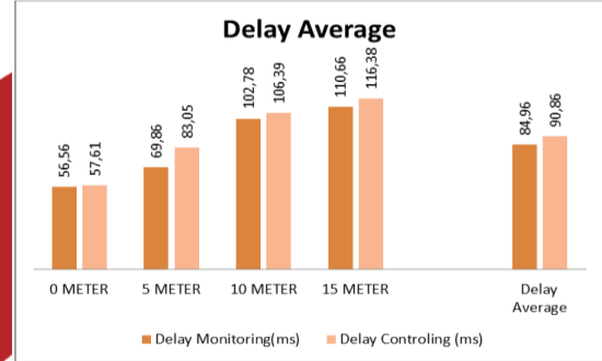
Figure 4.12 Average Total Delay
