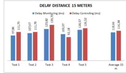
Figure 4.11 Delay measurement chart at 15 meters
