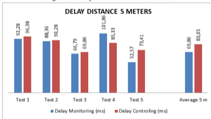
Figure 4.9 Delay measurement chart at 5 meters
