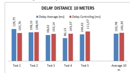
Figure 4.10 Delay measurement chart at 10 meters
