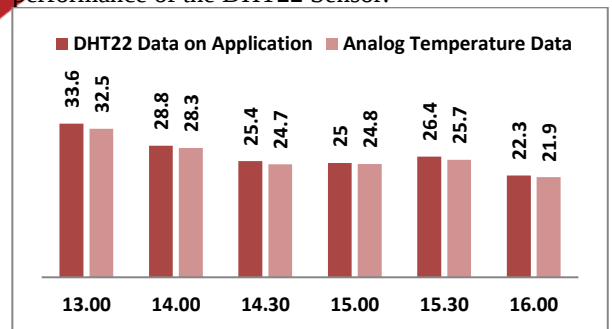
Figure 4.7. Temperature Value comparison chart
