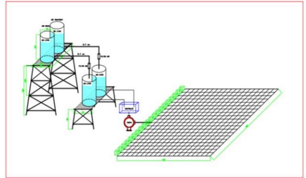
Figure 3.1. Drip Irrigation model realization
