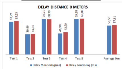
Figure 4.8 Delay measurement chart at 0 meters
